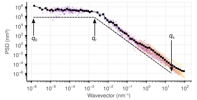
Fig. 5. Canonical model of the power-spectral density (PSD) used in many theoretical works (black line), with a constant PSD from system size at wavevector q_0 to the roll-off at wavevector q_r , where the PSD crosses over to a power law at short wavelength. The power-law region often extends down to the atomic scale, described by the short-wavelength cutoff q_s . For a self-affine topography, the power-law region follows the scaling q^{-1-2H} for the one-dimensional ( D = 1 ) PSDs shown here, where H is the Hurst exponent. The data shown is from a measurement of a microcrystalline diamond film that exhibits this idealized PSD. Black circles show the average over all individual measurements, shown by crosses. The roll-off wavelength 2\pi/q_r \approx 1 \mu\text{m} corresponds to the film thickness. The experimental data (different colors refer to individual measurements) is taken from Ref. [130].
