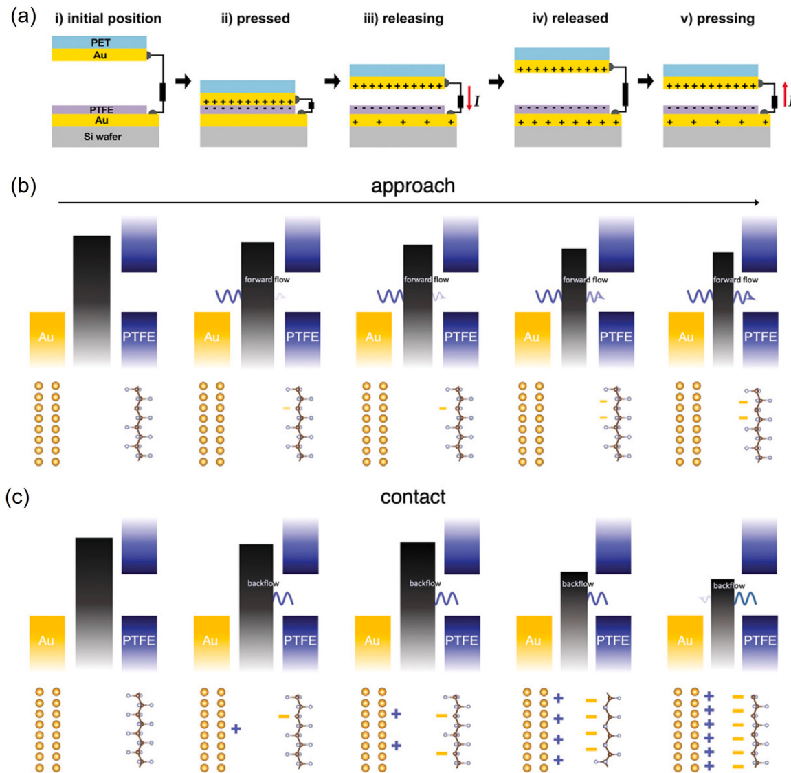
Fig. 15. Schematics of working principle and possible governing mechanisms of contact-separation (CS) mode TENGs. (a) Diagram of the pushing/releasing mechanism to generate the triboelectric signal. The proposed working principles of a PTFE/Au CS TENG are also depicted: during approach (b) the electrostatic barrier lowers and enables the forward flow of electrons; during the contact stage (c) charging is governed by the competition between the larger electron transfer prompted by an increasing defluorination and a backflow generated by a smaller interface separation. Reprinted from [437], licensed under CC-BY 4.0.
