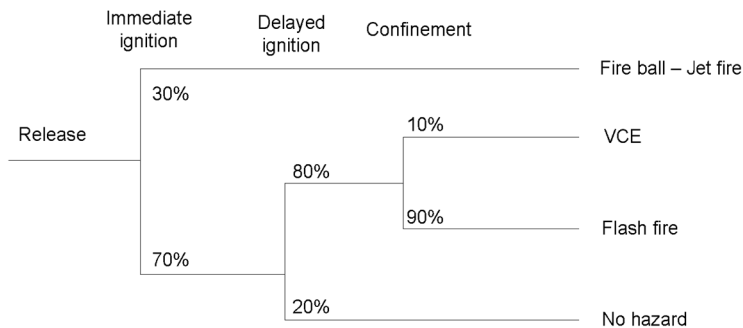
Figure 1. Event tree scheme adopted for pipelines components.
