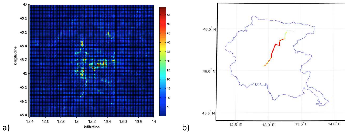
Figure 3. Representation of the Mw 6.4 1976 Friuli earthquake peak ground velocity field #12 (a) and 95th percentile average consequence radius for the pipe #048 (b).
