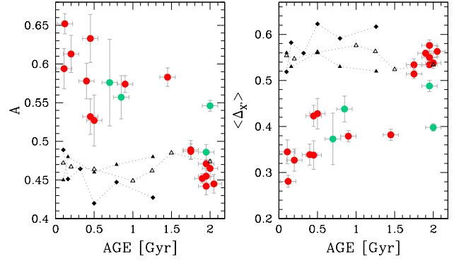
Fig. 15. Area below the \Delta_X cumulative curve, A , (left) and median \Delta_X value as a function of cluster age for LMC (red dots) and SMC (aqua dots) clusters with the eMSTO. Open and filled triangles are inferred from simulated CMDs of nonrotating stellar populations with different ages derived from the Padova and Geneva database, respectively. The diamonds correspond to coeval stellar populations with different rotation rates from the Geneva database. See text for details.
