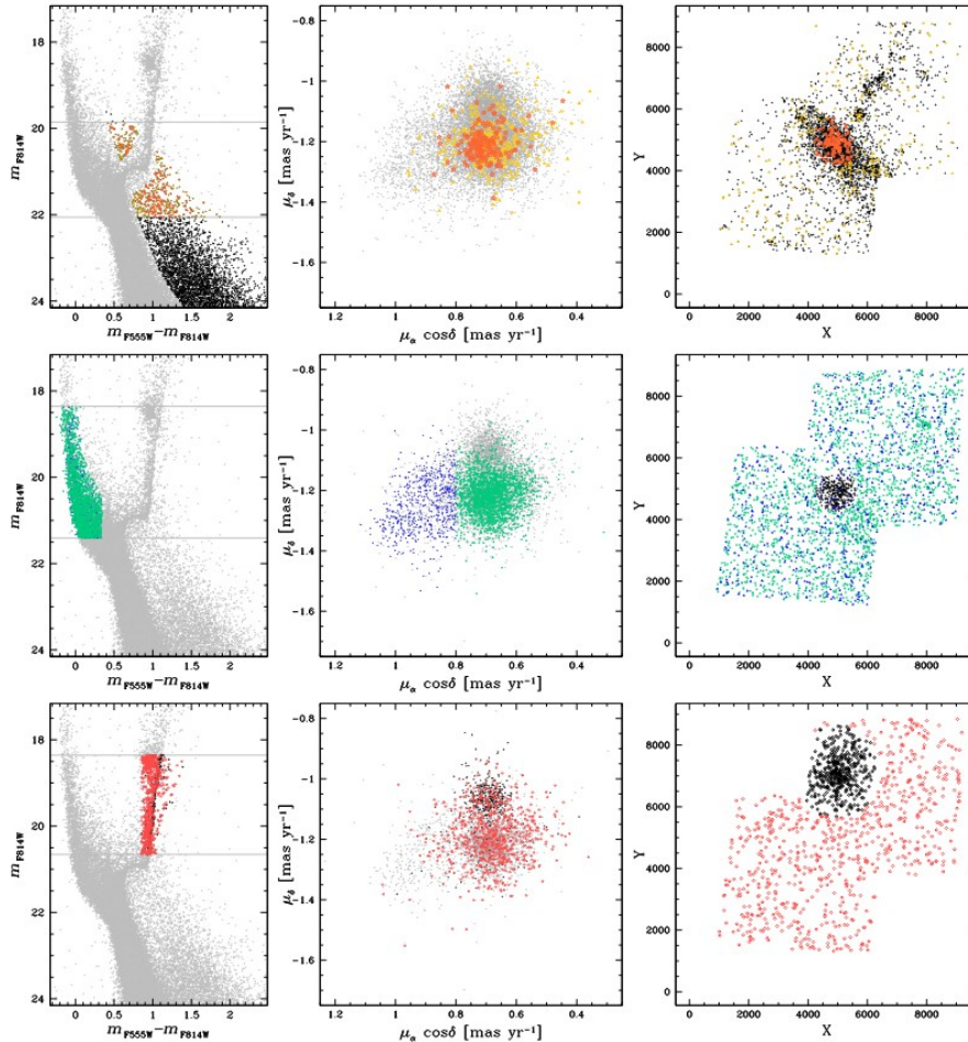
Fig. 25. Photometry, proper motions, and astrometry of the stellar populations in the field of view of NGC 346. The three left panels are reproductions of the m_{F814W} vs. m_{F555W} - m_{F814W} CMDs for stars in the field of view of NGC 346 and are used to select various groups of stars that we represented with colored symbols. The middle panels show the proper motions for stars in the magnitude interval delimited by the horizontal lines in the corresponding CMDs, whereas the right panels show the coordinates of the selected stars. The top panels are focused on candidate pre-MS stars. Specifically, bright pre-MS within 28 arcsec from the center of NGC 346 (pre-MS I sample) are represented with orange symbols, the remaining bright pre-MS stars (pre-MS II sample) are colored yellow, while the black symbols in the top panels mark faint pre-MS stars. Bright MS stars are investigated in the middle panels. Blue and aqua colors mark MS I and MS II stars, which have radial distances larger than 28 arcsec from the center of NGC 346, but different proper-motion distributions. The remaining bright-MS stars are colored black. The bottom panels highlight the selected RGB stars with radial distances from the center of BS 90 larger (red) and smaller than 60 arcsec (black).
