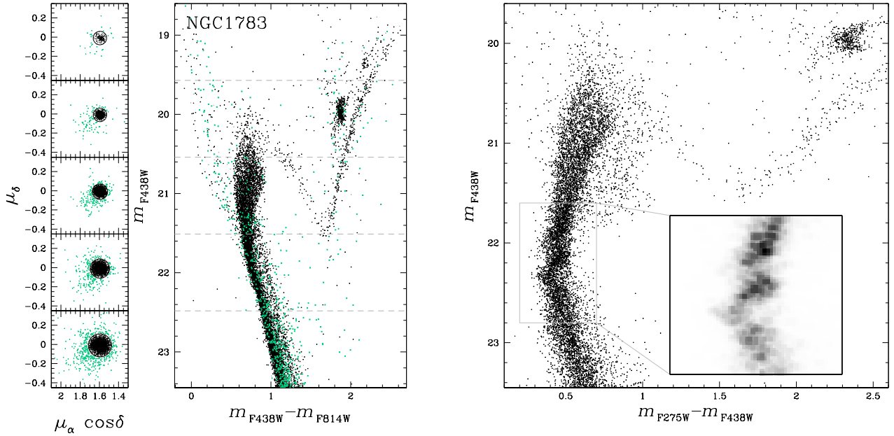
Fig. 16. Proper-motion diagrams of stars in the field of view of NGC 1783 in five F_{438W} magnitude intervals ( left ). The m_{F_{438W}} vs. m_{F_{438W}} - m_{F_{814W}} CMD for stars in the left panels is plotted on the middle . Stars within the black circles plotted in the proper-motion diagrams are considered probable cluster members and are colored black, whereas field stars are represented with aqua crosses. The right panel shows the m_{F_{438W}} vs. m_{F_{275W}} - m_{F_{438W}} CMD for probable cluster members, while the inset represents the Hess diagram of the CMD region around the upper MS.
