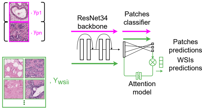
Fig. 1. Overview of the training schema for the multi-task Multiple Instance Learning CNN. The framework adopted is an instance-based MIL (the CNN produces predictions at both patch- and image-level).
