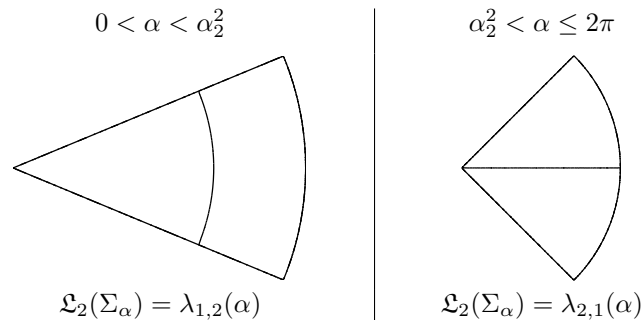
FIGURE 3. Minimal 2-partition on \Sigma_\alpha .
