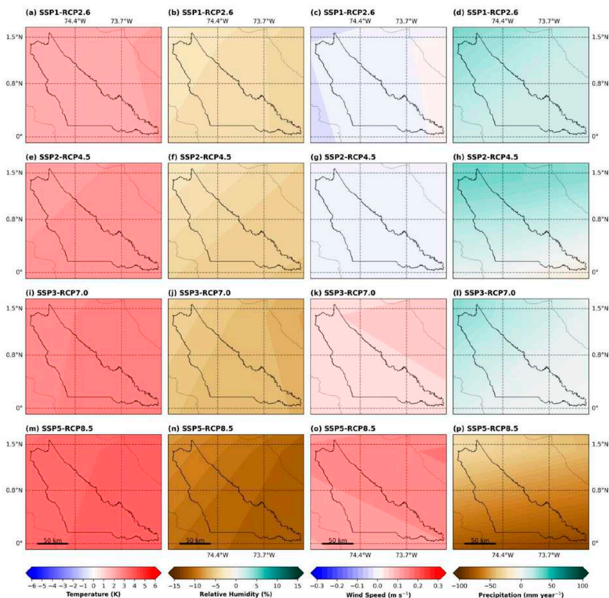
Figure 11. Climatological anomalies between the near-future and the historical period for boreal summer for (a,e,i,m) the surface air temperature, (b,f,j,n) surface RH, (c,g,k,o) surface wind speed, and (d,h,l,p) precipitation. Additionally, each row represents a different scenario: (a–d) SSP1-RCP2.6, (e–h) SSP2-RCP4.5, (i–l) SSP3-RCP7.0, and (m–p) SSP5-RCP8.5. The plot was constructed using the Cartopy Python package [81].
