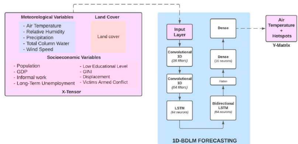
Figure 2. Neural network structure. Every box has the number of neurons/filters in the layer. The dropout percentage of a layer is also indicated. Notice that the purple boxes include the variables that construct the X-tensor and the Y-matrix.
