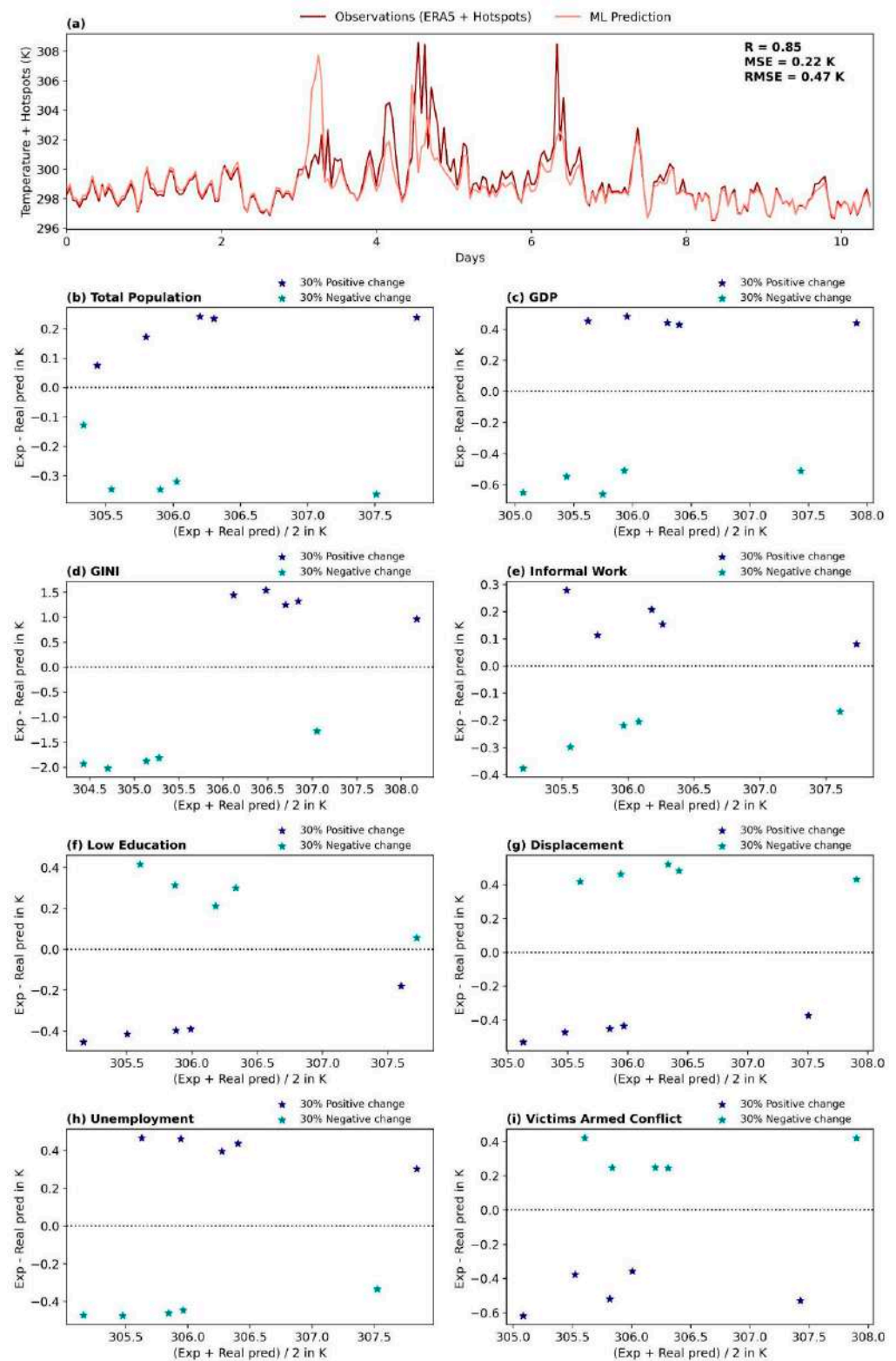
Figure 12. (a) ML model evaluation of three months of data. Here, a subset of 10.5 days that includes wildfires is plotted. Notice that the R, MSE, and RMSE are also plotted in the figure but are calculated for the three months and not only for the subset. Bland–Altman plots for experiments increasing (blue stars) and decreasing (green stars) by 30% the socio-economic variables: (b) total population, (c) GDP, (d) GINI, (e) informal work, (f) low education level, (g) displacement, (h) unemployment, and (i) victims armed conflict. For plotting purposes, each star represents the mean of 10 wildfire events that present similar temperatures.
