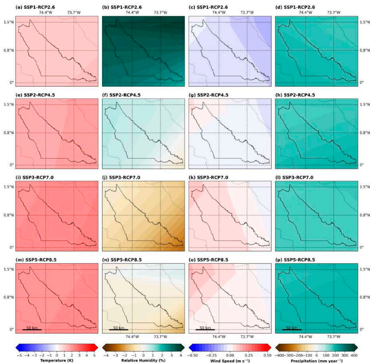
Figure 10. Climatological anomalies between the near-future and the historical period for boreal-winter for (a,e,i,m) the surface air temperature, (b,f,j,n) surface RH, (c,g,k,o) surface wind speed, and (d,h,l,p) precipitation. Additionally, each row represents a different scenario: (a–d) SSP1-RCP2.6, (e–h) SSP2-RCP4.5, (i–l) SSP3-RCP7.0, and (m–p) SSP5-RCP8.5. The plot was constructed using the Cartopy Python package [81].
