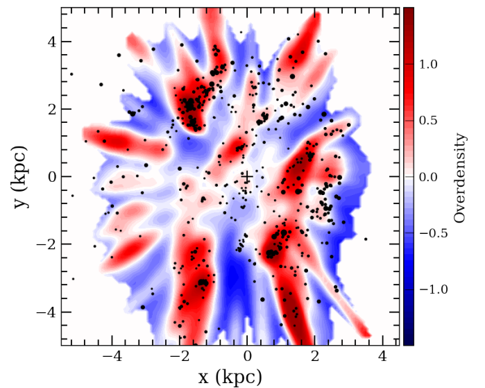
Fig. 13. Overdensity map of the OB stars overplotted with the positions of the open clusters younger than 63 Myr and with n_0 > 5 , plotted with filled circles whose size is proportional to \sqrt{n_0} . The cross indicates the position of the Sun.
