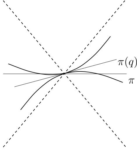
FIGURE 1. The region delimited by the thick curved lines is the right hand side of (6.10), whereas the cone delimited by the thick dashed straight lines is the right hand side of (6.8)
