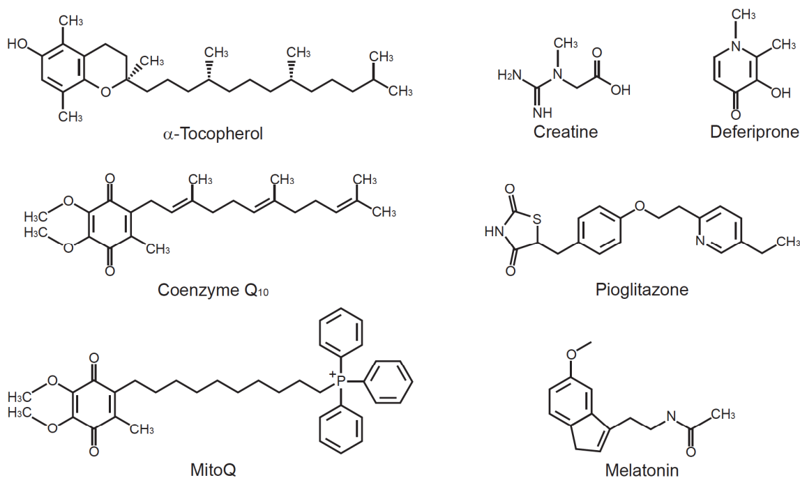
Fig. (2). Chemical structure of the antioxidant molecules described in the present paper.
