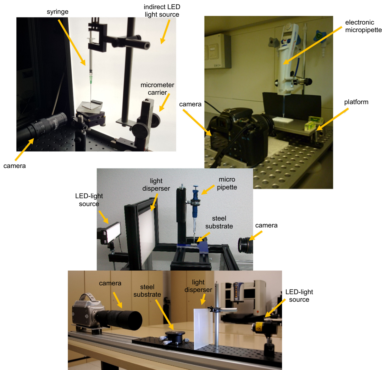
Fig. 3. In-house built contact angle measurement devices. Upper photos show the UJI device (left) and the NAITEC device. Middle photo represents the ILK device and lower photo the UoP device.
