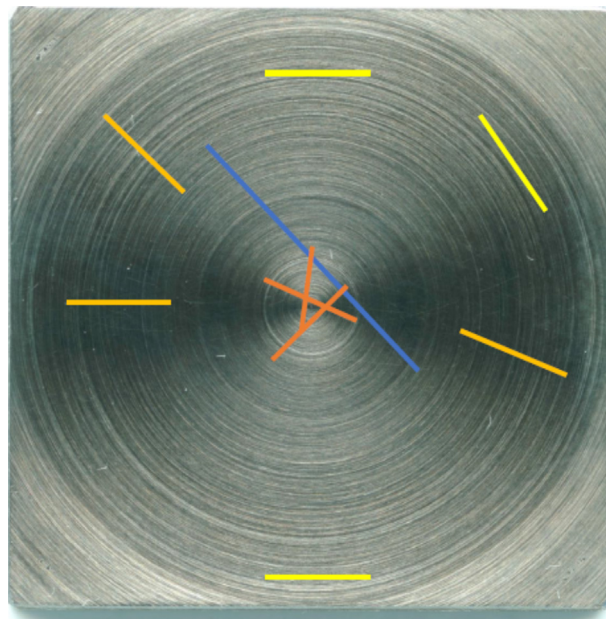
Fig. 2. Frontal view of stainless steel substrate. Droplets for CA measurements are placed right in the centre of the substrate. Lines indicate Perthometer path to measure surface roughness. For measured roughness values, see Table A2 of Supplementary Material.
