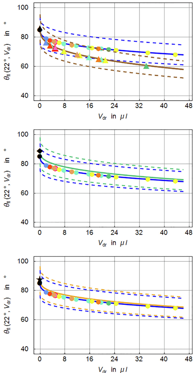
Fig. 8. Replot of experimental data employing the fitting functions for 22 °C. Upper graphene oxide (brown), middle plot alumina nanofluid (green), and lower plot gold nanofluid (yellow). Blue curves indicate water. Full curves show fit at 22 °C and broken curves \pm 10\% departure.
