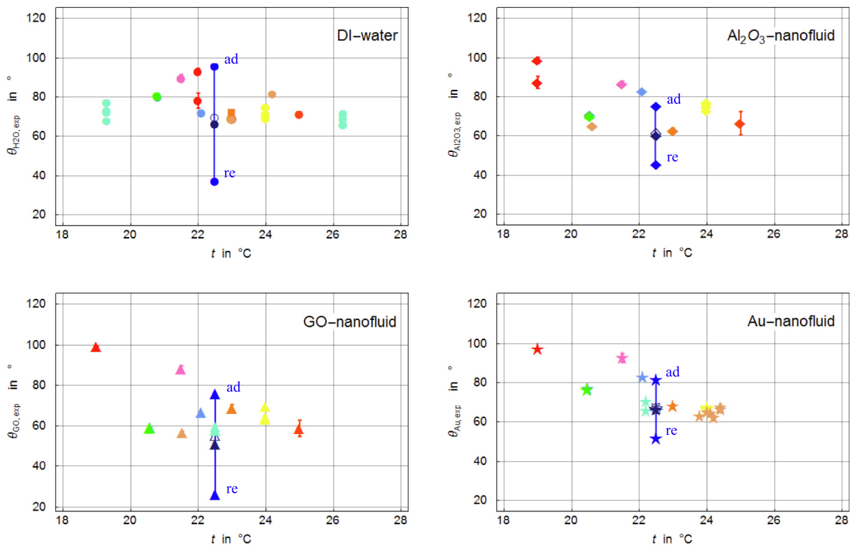
Fig. 6. Raw data of contact angle. Upper plot reference fluid DI-water and lower plot graphene oxide nanofluid. Wilhelmy plate results are connected by vertical lines. The arithmetic mean of advancing and receding CA are depicted by dark blue symbols and the arithmetic mean of their cosines with empty dark blue symbols. Raw data of contact angle. Upper plot shows alumina nanofluid and lower plot gold nanofluid.
