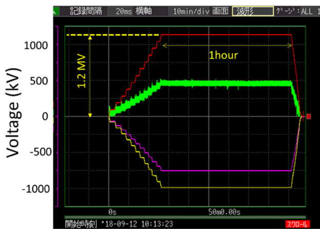
Figure 13. MITICA high-voltage test, first step: 1200 kV for 1 h.
