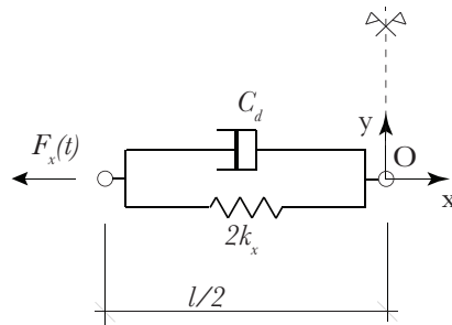
Fig. 14. Kelvin-Voigt model adopted to describe the viscoelastic behaviour of the DE actuator.
