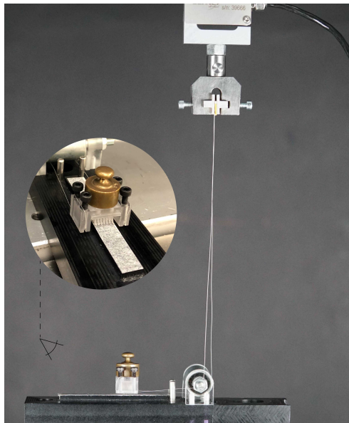
Fig. 7. Experimental setup for the measurement of the friction force generated at the interface between the testing surface and the bristle pads. The bristle pad sample coupled to the sample holder and loaded with a mass m = 20 g constituting the slider. A double inextensible wire allowed for pulling the slider with a tensile machine along the linear guide covered with a layer of baking paper showed in the enlargement of the picture.
