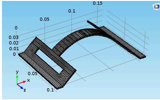
Fig. 13. Mesh of the robot plastic structure about the initial configuration of equilibrium. The DE actuator is not visually represented since its presence is imposed as equivalent spring constraints to the plastic structure.
