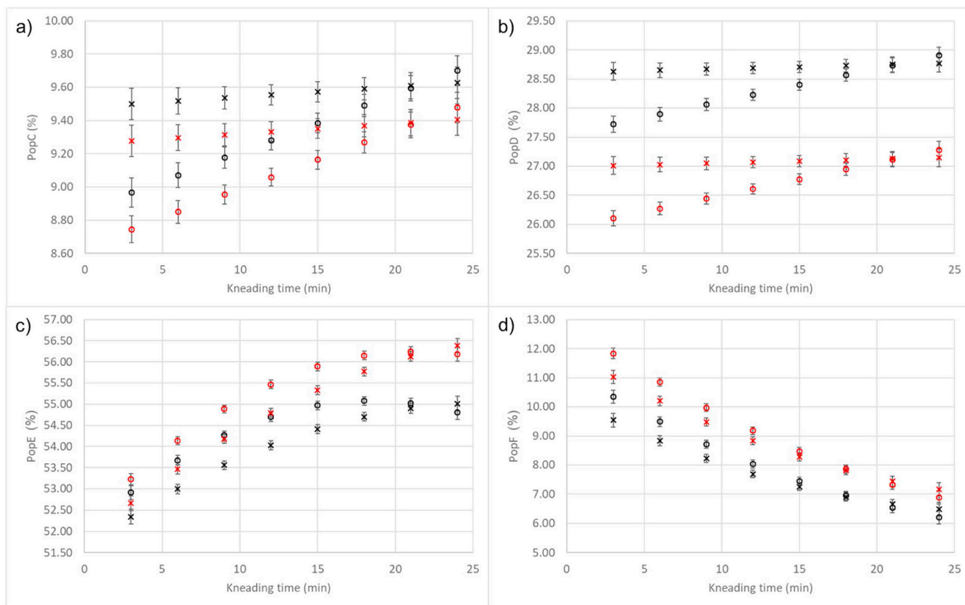
Fig. 2. Kinetic models of ^1\text{H} NMR proton populations in WWF doughs during kneading obtained from CPMG pulse sequence experimental data: a) relative abundance of population C (popC, %), b) relative abundance of population D (popD, %), c) relative abundance of population E (popE, %) and d) relative abundance of population F (popF, %). The symbol “o” represents FFT56:0 (control WWF dough at 56% water content), “x” FFT56:5 (WWF dough at 56% water content with gradual addition of 5% water during kneading) and “x” FFT60:5 (WWF dough at 60% water content with gradual addition of 5% water during kneading). The black bars represent the 95% confidence interval of the model.
