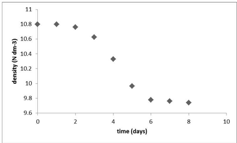
Figure 2: Measured density during the alcoholic fermentation as a function of time.
