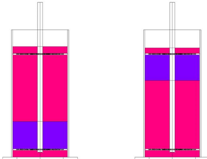
Figure 1: Representation of the two-plate measurement system. In the picture the juice is represented in red, while the cap in purple. The left picture shows the case of sank berries (negative force values), while the right picture the case of floating pomace cap (positive force values).
