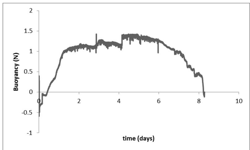
Figure 3: Recorded buoyancy of the pomace cap during the alcoholic fermentation.
