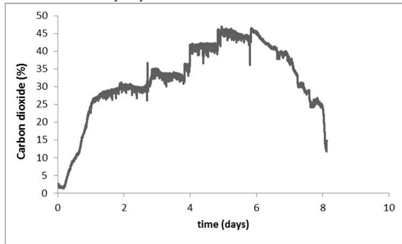
Figure 4: Calculated volume (%) occupied by the carbon dioxide in the pomace cap.
