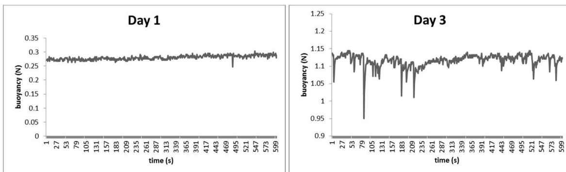
Figure 5: 10 min of buoyancy values recorded at day 1 and day 3.
