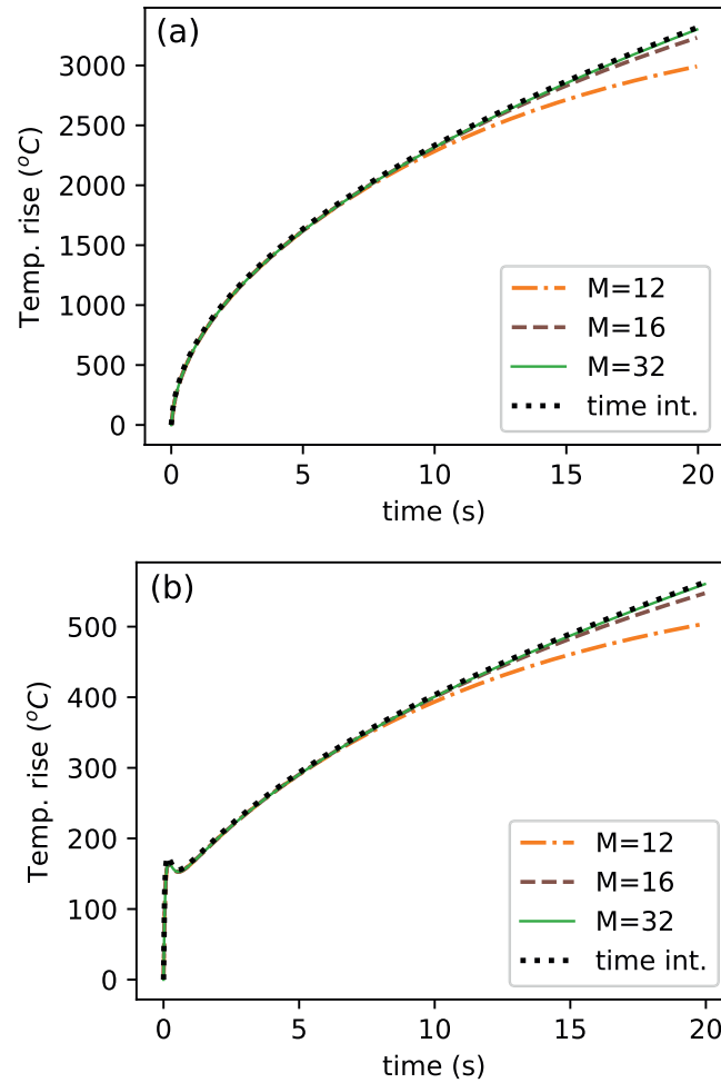
Figure A1. Test of the parsimonious scheme (wavenumber summation Equation A13). Temperature evolution is shown for (a) constant heat flux ( 3 \cdot 10^6 \text{ W m}^{-2} ) and (b) exponentially decaying heat flux ( 5 \cdot 10^5 + 3 \cdot 10^6 \exp(-10 t) ). Solutions are shown for M = 12, 16, 32 (dot-dashed, dashed, and solid curve, respectively). For comparison, the solution obtained from the direct discretization (Equation A2) of the analytical solution (time integral) is shown (dotted curve). The time-stepping is dt = 0.04 . See text for further details.
