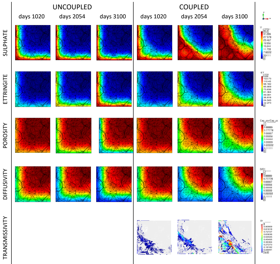
Figure 2: Results of the uncoupled and coupled analysis: contour plots on the upper face of specimen, of sulphate [ \text{mol/m}^3 ], ettringite [ \text{kg/m}^3 ], porosity, diffusivity and transmissivity [ \text{cm}^3/\text{day} ], all at three different times ( t = 1020, 2054 and 3100 days).
