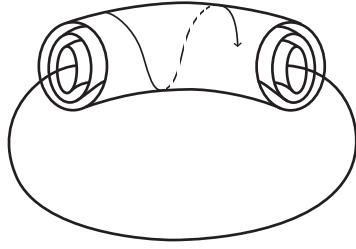
Figure 6. In classical mechanics, the Liouville–Arnol’d theorem establishes that, when enough conserved quantities in involution exist, the phase space is foliated in tori where the dynamics is supported. Here we depict such a foliation, with the arrow representing the motion of a particle.
