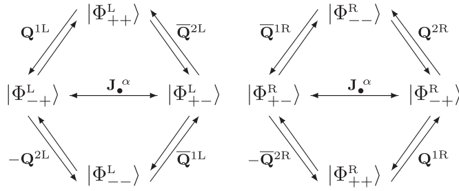
Figure 24. The action of the supercharges on the massive excitations is supplemented by J^\alpha from \mathfrak{su}(2)_\bullet , acting on the massive fermions only. Note that for clarity we only depict the action of some of the supercharges, i.e. the ones that remain non-trivial on-shell. [176] Reproduced with permission from Borsato R et al 2014 Phys. Rev. Lett. 113 131601. Copyright 2014 by the American Physical Society.
