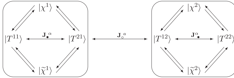
Figure 25. The massless excitations sit in two \mathfrak{psu}(111)_{\text{c.e.}}^4 modules, with fermionic highest weight states. The two modules transform as a doublet under \mathfrak{su}(2)_{\circ} , and additionally the bosons T^{aa} also carry a Greek index of \mathfrak{su}(2)_{\bullet} . [176] Reproduced with permission from Borsato R et al 2014 Phys. Rev. Lett. 113 131601. Copyright 2014 by the American Physical Society.
