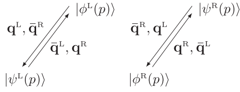
Figure 5. The action of the supercharges \mathbf{q}^{L,R} and \bar{\mathbf{q}}^{L,R} of \mathfrak{psu}(111)_L \oplus \mathfrak{psu}(111)_R centrally extended on an arbitrary momentum (off-shell) excitation (2.102).
