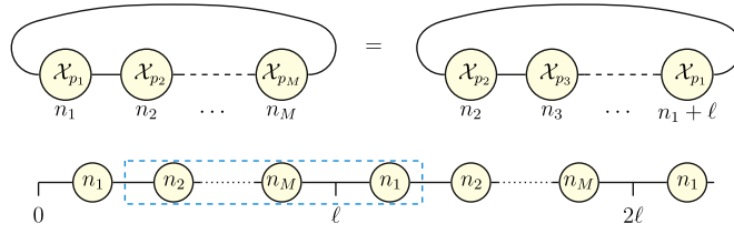
Figure 20. Illustrations of the periodicity condition leading to the Bethe ansatz equations. Above: the two ends of the chain have been identified, so that the first excitation \mathcal{X}_{p_1} in position n_1 can be thought as sitting at the end of the chain, in position n_1 + \ell . This can be realized by scattering \mathcal{X}_{p_1} through all of the \mathcal{X}_{p_j} . Below: equivalently, the wave-function should be \ell -periodic as a function on \mathbb{R} . The box identifies the periodicity condition evaluated as in (6.5).
