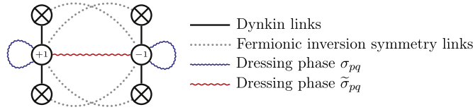
Figure 23. The Dynkin diagram for \mathfrak{psu}(1, 1|2)^2 with the various interaction terms appearing in the Bethe ansatz indicated. The label \pm 1 inside the middle Dynkin nodes indicate the \mathfrak{su}(2) and \mathfrak{sl}(2) gradings of the left- and right-moving sectors.
