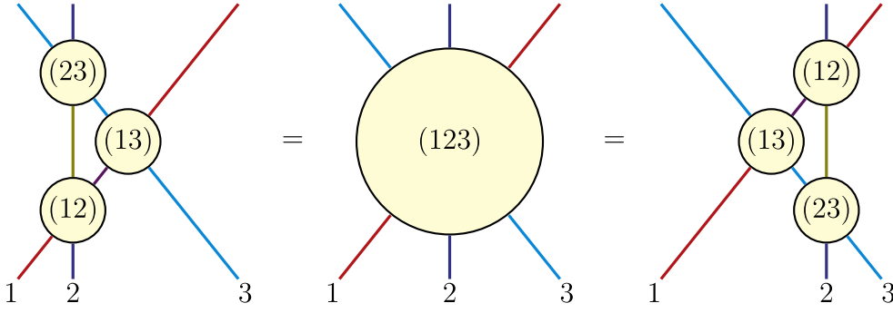
Figure 7. Different ways of resolving the 3 \rightarrow 3 particle scattering (central panel). The lines are colored in such a way as to allow for a non-trivial flavor structure, which may be affected by the scattering. Taking time to flow upwards, we have in the left panel the sequence of scattering (12)-(13)-(23), while in the right panel we have (23)-(13)-(12). The Yang–Baxter equation imposes the equality of the two resolutions.
