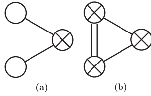
Figure 26. Two Dynkin diagrams for \mathfrak{d}(2, 1; \alpha) . Diagram (b) corresponds to a completely fermionic grading.
