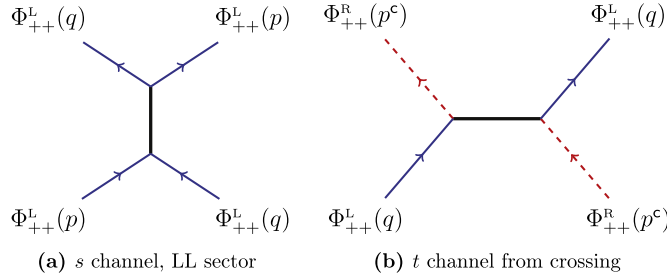
Figure 13. On the left two particles in the same sector form an \mathfrak{su}(2) bound state in the s channel. Applying the crossing transformation to \Phi_{++}^L(p) yields the t -channel diagram on the right, where one particle has unphysical momentum p^c (red dashed lines). [173] Reproduced with permission from Borsato R et al 2013 Phys. Rev. D 88 066004. Copyright 2013 by the American Physical Society.
