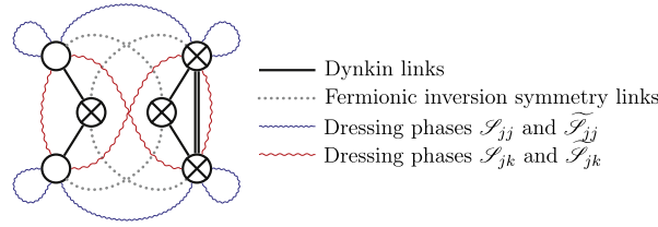
Figure 28. The Dynkin diagram for \mathfrak{d}(2, 1; \alpha)^2 in mixed grading (see figure 26), with the various interaction terms of the Bethe ansatz indicated. Note how now, besides dressing phases that couple nodes of the same mass (in blue), there appear phases coupling nodes of mass \alpha with ones of mass 1 - \alpha (in red).
