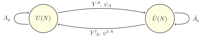
Figure 2. The quiver diagram of ABJM theory, where we have drawn an arrow from the fundamental to the anti-fundamental representation of each gauge group. Note that the scalars Y^A and the fermions \psi_A , as well as their conjugates, carry an index of the R-symmetry group SU(4) , A = 1, \dots, 4 .
