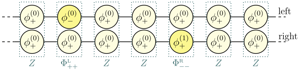
Figure 17. A pictorial representation of the \mathfrak{psu}(1, 1|2)^2 spin chain. We can think of it as two (left and right) spin chains, each with ground state \phi_+^{(0)} . Excitations of the whole chain are considered as left- or right- moving depending on whether we excite a spin in the left or right chain.
