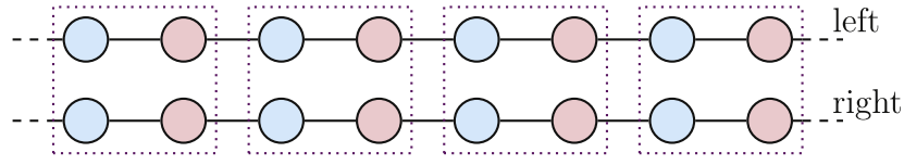
Figure 27. Pictorial representation of the \mathfrak{d}(2, 1; \alpha)^2 alternating spin chains. We can think of it as composed of two (left and right) alternating chain. For each of these, odd (cyan) sites are in the (\frac{\alpha}{2}; \frac{1}{2}; 0) representation of \mathfrak{d}(2, 1; \alpha) , while even (pink) sites are in the (\frac{1-\alpha}{2}; \frac{1}{2}; 0) representation. The dotted squares represent the combination of sites which we identify as fundamental excitations of the whole \mathfrak{d}(2, 1; \alpha)^2 chain.
