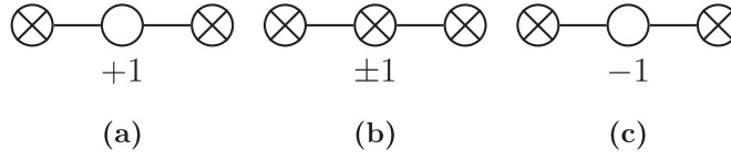
Figure 22. Three Dynkin diagrams for \mathfrak{psu}(1, 1|2) . From left to right, we depict the \mathfrak{su}(2) grading, two fully fermionic gradings and the \mathfrak{sl}(2) grading.
