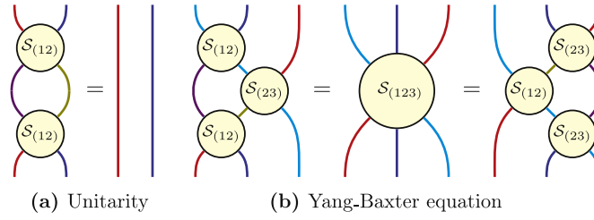
Figure 18. Consistency conditions on the spin-chain S matrix. Unitarity (left panel) requires that acting twice with S_{(12)} on a two-particle state gives back the original state. The Yang–Baxter equation (right panel) resolves the ambiguity in decomposing the scattering of three excitations. Note how, with respect to figure 7, this picture takes into account how S permutes the spin-chain excitations.
