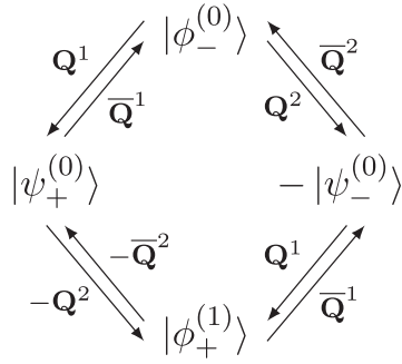
Figure 16. The action of the supercharges Q^j = Q^{jL,R} and \bar{Q}^j = \bar{Q}^{jL,R} on the either of the left- or right-bifundamental representation (5.17). It takes the same form of figure 4.
