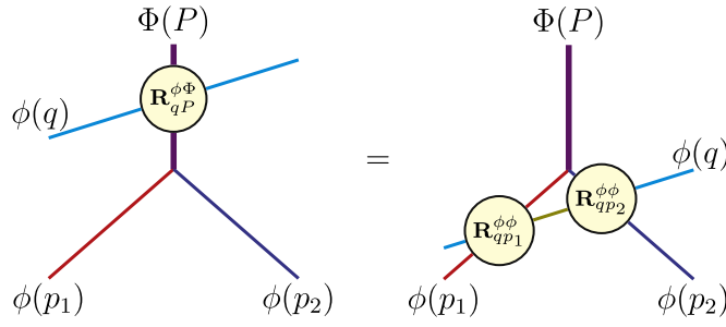
Figure 9. The bootstrap condition for the bound-state S matrix. We consider two particles \phi with complex momenta p_1 = \frac{1}{2}P + iv and p_2 = \frac{1}{2}P - iv that form a bound state \Phi of momentum P (thicker violet line). The scattering of a third particle \phi(q) with \Phi(P) can be resolved in terms of the scattering with its constituents. Note that the point in the diagram at which the two particle fuse to give a bound state should not be interpreted as a scattering event.
