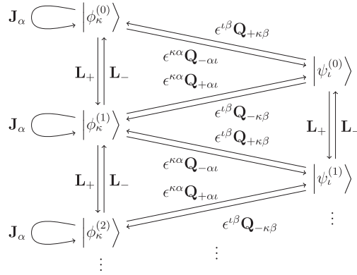
Figure 15. An illustration of the short \left(\frac{1}{2}; \frac{1}{2}\right) module, where the action of the (super) charges is represented up to the numerical coefficients. These are given in equation (5.4)–(5.6).
