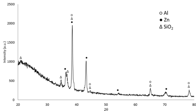
Figure 4. XRD analysis of the sample obtained at 2.3 A/cm 2 for 2 min.
