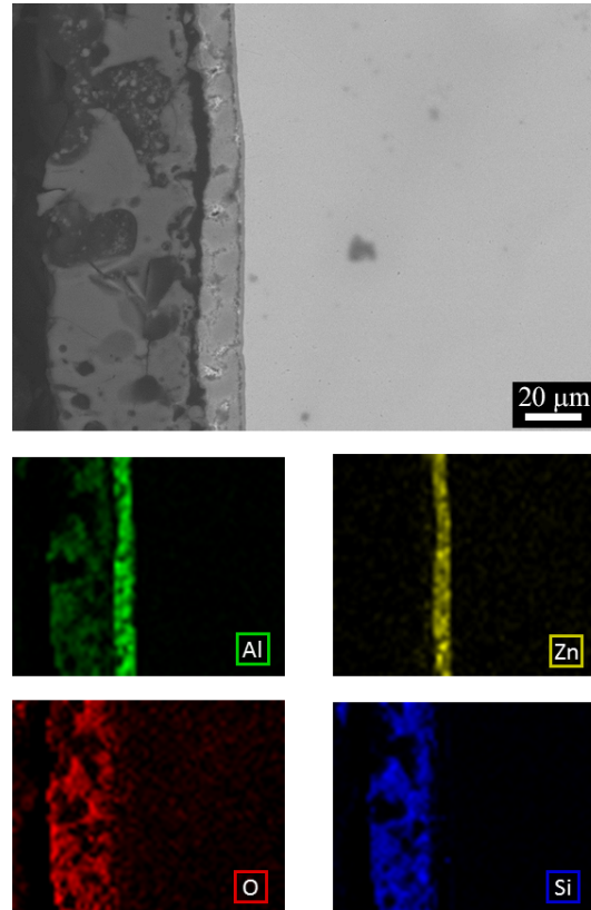
Figure 3. SEM-EDS elemental mapping performed on the cross section of the sample obtained at 2.3 A/cm 2 for 2 min.
