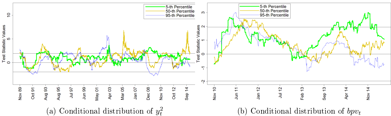
Figure 11: The Diebold and Mariano (2002) test statistic values over the rolled windows. Subfigures 11(a) and 11(b) refer, respectively, to the forecasts of the y_t^2 and the bpv_t distributions, where we compared the restricted (which contain just the lags of y_t^2 and bpv_t ) and the unrestricted models (which include also the lags of x_{1,t} and x_{2,t} ). The test was applied for three different \tau values: 0.05 (green lines), 0.50 (yellow lines) and 0.95 (blue lines). The black horizontal lines represent the 5% confidence bounds.
