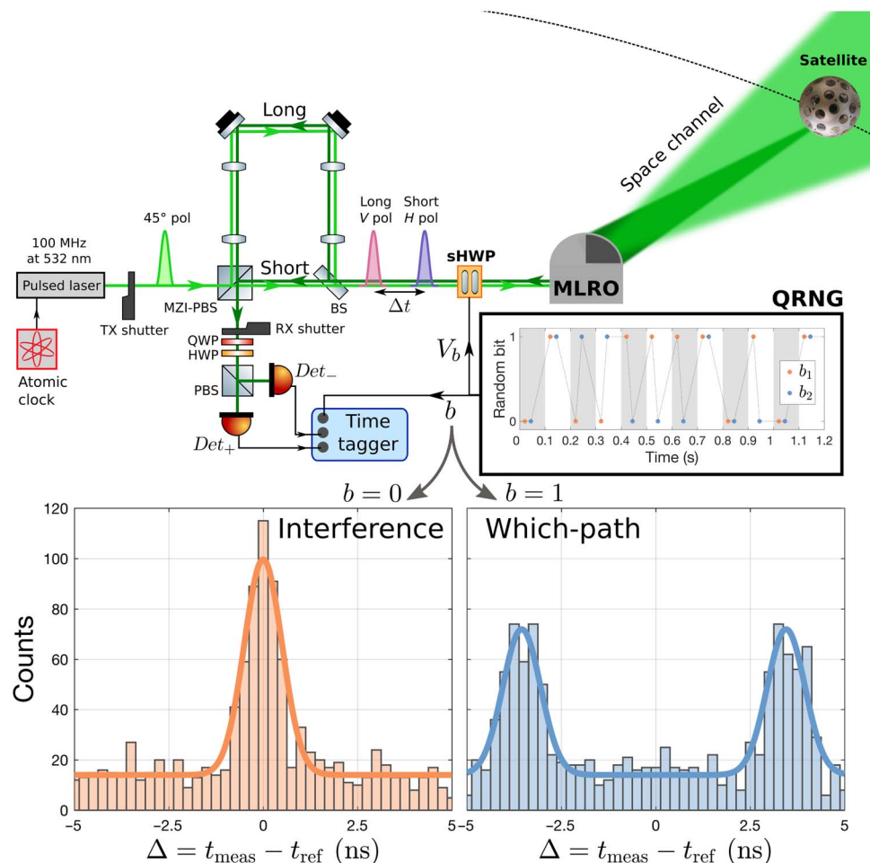
Fig. 2. Scheme of the experimental setup and detection histograms. A pulsed laser synchronized with the MLRO atomic clock exits the MZI in two temporal and polarization (pol) modes. The sHWP leaves the pulses unperturbed, and the telescope directs the beam to a target satellite. After the reflection, the photons are collected on the ground by the same telescope and injected into the optical table. The photons pass through the sHWP whose behavior is set according to the bit b extracted from an on-demand QRNG. The QRNG is inquired twice in each 100-ms cycle of the experiment, as detailed in the main text. In the inset, a 1-s sample of the extracted bits is shown. At the MZI output, two wave plates, a PBS, and two single-photon detectors (SPDs) perform a polarization measurement in the \{|+\rangle, |-\rangle\} basis. According to the value b of the random bit, interference or which-path measurement is performed, as shown by the detection histograms for a passage of the Starlette satellite. The counts in the central peak on the left histogram are comparable to the sum of the counts associated to the lateral peaks on the right one, as expected. HWP, half-wave plate; QWP, quarter-wave plate.
