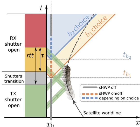
Fig. 3. Minkowski diagram of the experiment. Along the temporal axis (not to scale) a 100-ms cycle between two SLR pulses is represented. The x axis represents the radial coordinate (not to scale) from the detectors, where x_0 is the position of both the sHWP and the QRNG. The dotted line is the satellite worldline. We only considered the detections in the temporal window \tau , as detailed in the main text. A fast FPGA controller synchronized in real time with the MLRO tracking system drives the two shutters and the QRNG. For each cycle, we performed two independent measurements via the random bit extracted by the QRNG at times t_{b_1} and t_{b_2} , causally disconnected from the photon reflection at the satellite. The cycle is repeated for each 100-MHz train between two SLR pulses.
