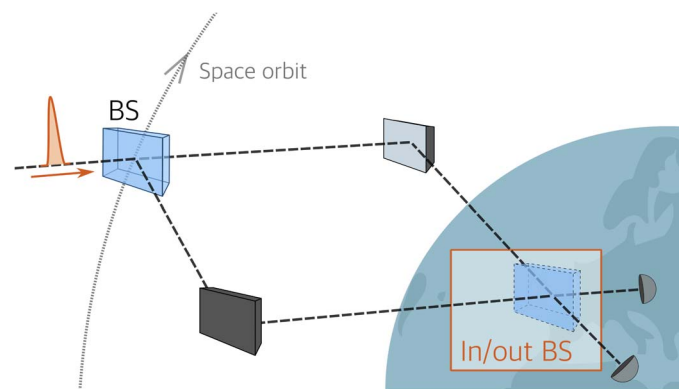
Fig. 1. Pictorial representation of Wheeler's delayed-choice experiment in space. A photon wave packet enters the first BS of an interferometer, which extends along thousands of kilometers in space. The interferometer can be randomly arranged according to two configurations that correspond to the presence or absence of the second BS (in/out BS) located on Earth. Following Wheeler's idea, the configuration choice is performed when the photon has already entered the interferometer. In our actual implementation, the interferometer begins and terminates on the ground, extending up to the target satellite, and the measurement choice performed on ground is space-like separated from the photon reflection by the satellite.
