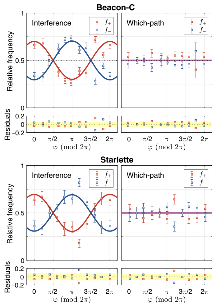
Fig. 4. Experimental results for the interference and which-path configurations. Relative frequencies f_{\pm} of counts in the two detectors \text{Det}_{\pm} as a function of the kinematic phase \varphi introduced by the satellite for the passages of Beacon-C and Starlette satellites. The error bars are estimated using the Poissonian error associated to counts. We show the relative residuals as a function of \varphi below each plot. We note that, at the point \varphi \approx 0 and \varphi \approx 2\pi , the same subset of data was selected. In the interference configuration, we estimated a visibility \mathcal{V}^B = 40 \pm 5\% for Beacon-C and \mathcal{V}^S = 39 \pm 4\% for Starlette from the fitted data.
