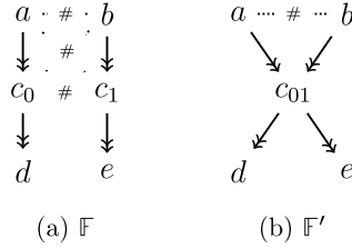
Fig. 12. A FES and a corresponding folding.
