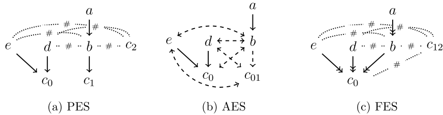
Fig. 1. Three history preserving bisimilar event structures.
