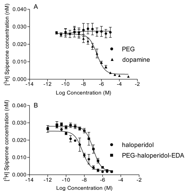
Fig. 4 Binding curves for compounds competing with [ 3 H] spiperone in D 2 receptors from CHO cells: (a) PEG, negative control and dopamine, positive control, (b) PEG-haloperidol and free haloperidol. Data expressed as the mean \pm SEM, ( n = 3 ). pK_i values were derived from data fitted to a single-binding site model.
