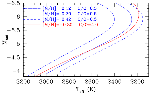
Figure 6. TP-AGB Hayashi lines for a model with M = 1.4 M_{\odot} at varying initial metallicity ( [M/H] ) and surface C/O ratio, as indicated. At a given bolometric magnitude, the effective temperature is obtained from integrations of complete atmosphere and envelope models (Marigo et al. 2013) that include on-the-fly computation of both molecular chemistry and opacity (Marigo & Aringer 2009). (A color version of this figure is available in the online journal.)
