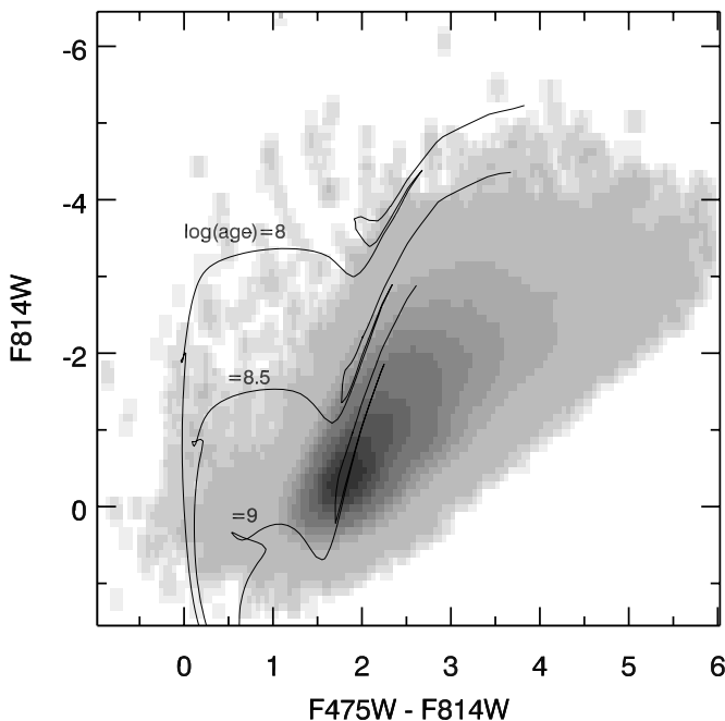
Figure 7. Optical CMD of the observed region, from the PHAT program (Dalcanton et al. 2012a). Padova isochrones are plotted with A(V) = 0.3 mag for \log(\text{age}) = 8, 8.5, \text{ and } 9 (PARSEC, version 1.1; Marigo et al. 2008; Girardi et al. 2010). The CMD indicates the presence of main sequence turn-off stars at least as young as \sim 300 Myr (or M \lesssim 4 M_{\odot} ).
