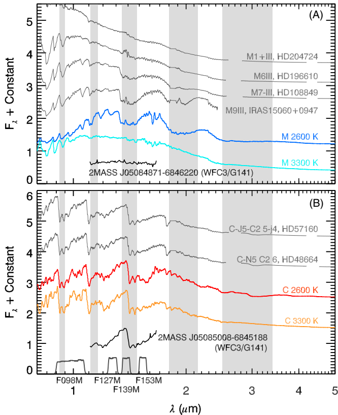
Figure 4. IRTF spectra of Galactic stars (Rayner et al. 2009), plotted in gray, for (A) M stars in order of increasing water absorption and (B) C stars. Solar metallicity model spectra from Aringer et al. (2009) and B. Aringer et al. (in preparation) are also plotted for (A) M stars (blue/cyan) and (B) C stars (red/orange) with T_{\text{eff}} = 2600 K and 3300 K. Shaded regions mark wavelengths affected by telluric absorption. The model spectra predict all major features present in the IRTF spectra. Also shown in black are telluric-free spectra of two stars in NGC 1850 across the spectral region covered by the WFC3/IR G141 grism: panel (A) shows the M star 2MASS J05084871–6846220 and panel (B) shows the C star 2MASS J05085008–6845188. These two stars present 2MASS colors and magnitudes typical of most C-rich and O-rich AGB stars in the LMC and do not show any surprising features in the F139M band.
