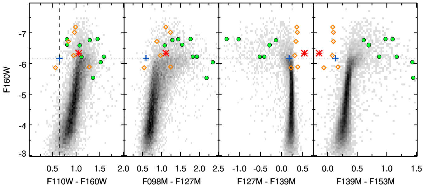
Figure 3. Color–magnitude diagrams, plotted as Hess diagrams to show the point-source density. F160W and F110W magnitudes come from the PHAT survey (Dalcanton et al. 2012a). Sources with H - K > 0.4 mag from Davidge et al. (2005) are plotted as large green circles. The horizontal dotted line is the F160W TRGB from Dalcanton et al. (2012a). The one carbon star candidate identified in Figure 5 is shown as a red asterisk, and the six sources that fall on the edge of the region covered by the carbon star models in Figure 5 are plotted as orange diamonds. An additional star on the edge of M star model coverage in Figure 5 is plotted as a blue plus symbol. This star has colors consistent with a foreground M dwarf (dashed line; also see Figure 21 from Dalcanton et al. 2012a), as does one of the C star candidates.
