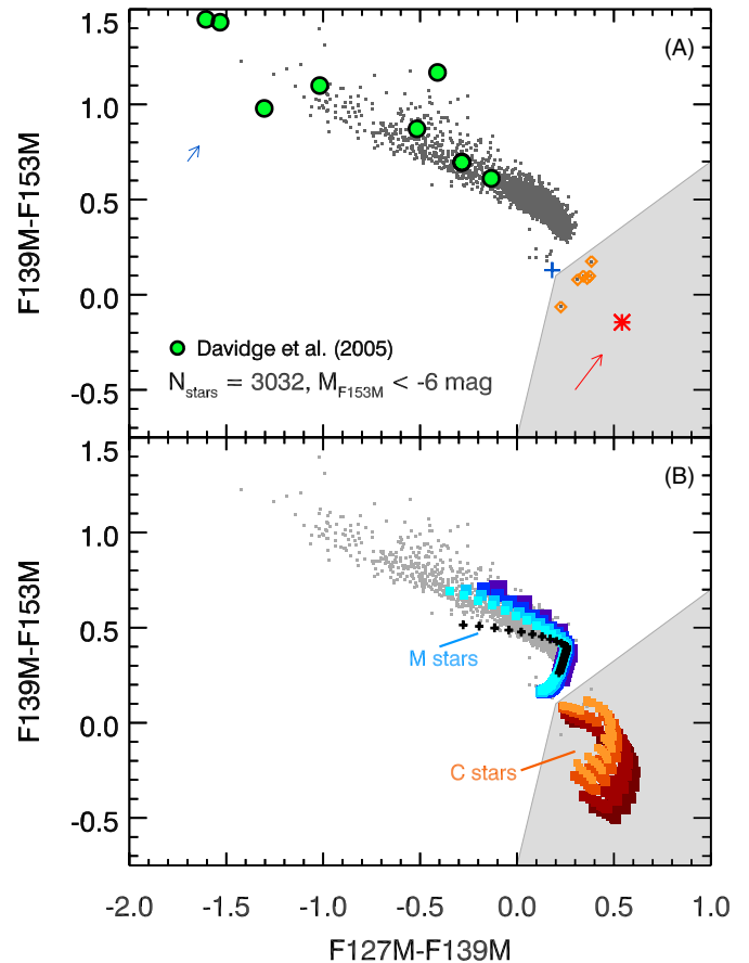
Figure 5. Color-color diagram comparing the WFC3/IR colors to the model predictions for C and M giants. Panel (A) shows the observed colors of AGB stars, with red stars from Davidge et al. (2005) plotted as green circles and candidate C stars marked as in Figure 3. Only stars brighter than the TRGB ( M_{F153M} < -6 mag) are included to eliminate most red giant branch stars. Circumstellar reddening vectors for dust-enshrouded stars are plotted with blue (M star) and red (C star) arrows for E(J - K_s) = 1.0 mag (corresponding to a mass-loss rate of \approx 10^{-6} M_{\odot} \text{yr}^{-1} ). These vectors are derived from Groenewegen (2006b) radiative transfer models applied to cool M and C stellar spectra, with 60% silicate + 40% AlOx, and 70% amorphous carbon + 15% SiC mixtures, respectively (see Marigo et al. 2008). In panel (B), AGB star models are plotted over the data. The M star models (B. Aringer et al., in preparation) are plotted as blue boxes (using the water line list from Jørgensen et al. 2001), with darker colors representing lower surface gravity, in the range 2 \geq \log g [\text{cm s}^{-2}] \geq -0.5 . The T_{\text{eff}} decreases from bottom to top along this sequence, with values in the range 5000 \leq T_{\text{eff}} \leq 2600 K: the kink with the reddest F127 – F139M colors is at T_{\text{eff}} \approx 3300 K. For reference, black pluses show an example of the same M star models ( \log g = 0.5 [\text{cm s}^{-2}] ) using a different water line list (Barber et al. 2006). The C star models (Aringer et al. 2009) are plotted as red boxes, with darker colors representing higher atmospheric C/O ratios, over the range 1.05 < C/O < 2 . They span 4000 \text{ K} \leq T_{\text{eff}} \leq 2400 \text{ K} and 0 \geq \log g [\text{cm s}^{-2}] \geq -1 , with the coolest C star models now being located at the bottom of the drawn sequences. All models assume a solar abundance for the heavy metals. The shaded region marks the area where C stars are expected.
