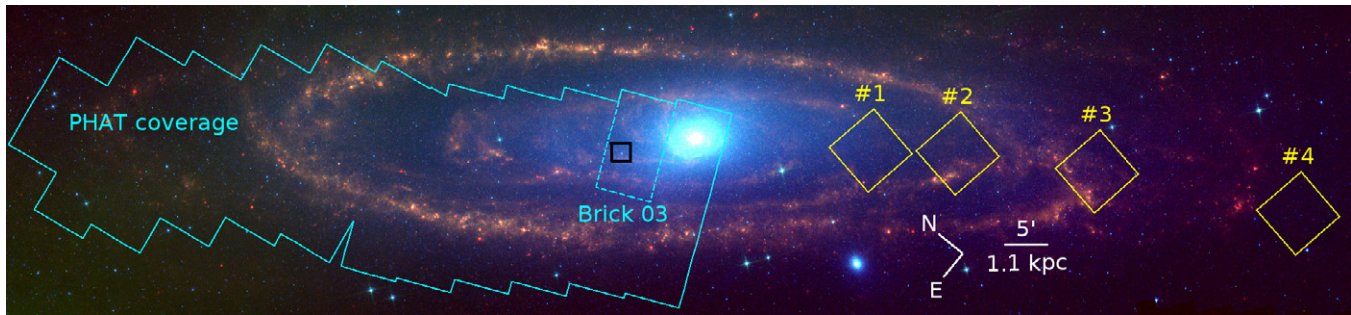
Figure 2. Three-color image of M31 from Spitzer (Barmby et al. 2006). 24\ \mu\text{m} is plotted in red, 5.8\ \mu\text{m} in green, and 3.6\ \mu\text{m} in blue. The PHAT coverage is shown in cyan (Dalcanton et al. 2012a). The coverage discussed here is shown in black and is part of the PHAT survey’s “Brick 03.” Four of the regions from Brewer et al. (1995) plotted in Figure 1 are shown in yellow. Region #5 is off the image to the southwest.
