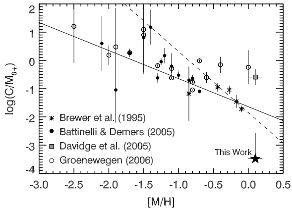
Figure 1. The C/M ratio, adapted from Groenewegen (2006a) and Battinelli & Demers (2005) for nearby galaxies. Data for five regions in M31 from Brewer et al. (1995) are plotted with asterisks, with metallicities from Zurita & Bresolin (2012). These data were derived using optical photometry, so the number of C stars is underestimated by \approx 20\% – 60\% (e.g., Boyer et al. 2009). The error bars are derived solely from Poisson statistics and do not include information on detection biases or photometric uncertainties. The solid line is fit through all points, and the dashed line is fit only through the Brewer et al. (1995) points. The Davidge et al. (2005) point (gray square) and the point from this work (star) are derived from NIR photometry, with the metallicity range from Saglia et al. (2010). We note that the metallicities for M31 are not measured directly for the fields included here, but are instead derived from estimates of the metallicity gradient across the disk (Zurita & Bresolin 2012) or the bulge (Saglia et al. 2010).
