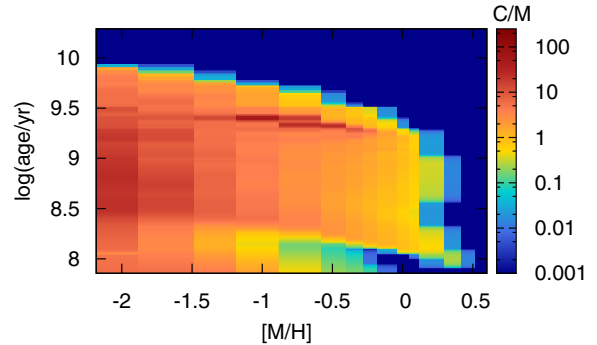
Figure 8. Map of the C/M ratio in the age–metallicity plane, according to the new TP-AGB models computed by Marigo et al. (2013). The lack of the C star phase ( C/M = 0 ) corresponds to the darkest blue region, which extends toward younger ages at increasing metallicity. Above some critical value of [M/H] , models predict C/M = 0 over the entire age range. According to Saglia et al. (2010), the metallicity of the region observed here is [M/H] \approx 0.1 \pm 0.1 . (A color version of this figure is available in the online journal.)
