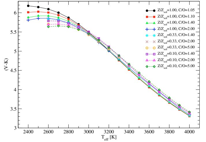
Fig. 13. Predicted (V-K) colours as a function of effective temperature calculated from COMARCS models with \log(g) [ \text{cm/s}^2 ] = 0.0, M/M_{\odot} = 2.0 and different values of Z/Z_{\odot} (denoted as Z/Z_{\text{sol}} in the plot) and C/O .
