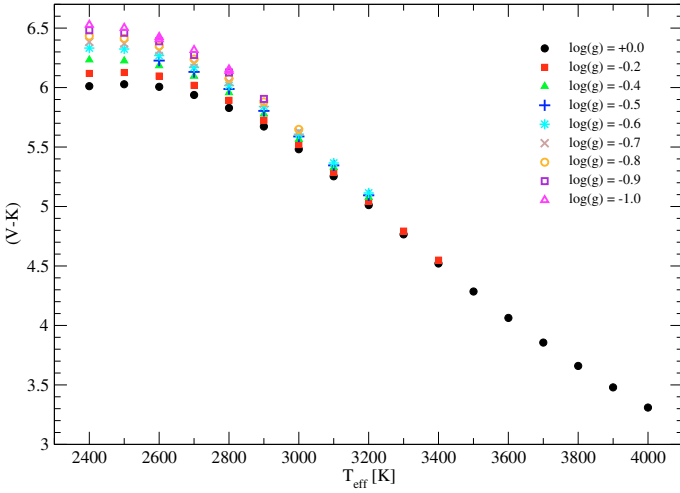
Fig. 12. Predicted (V-K) colours as a function of effective temperature calculated from COMARCS models with Z/Z_{\odot} = 1.0 , M/M_{\odot} = 2.0 , C/O = 1.10 and different values of \log(g) [ \text{cm/s}^2 ].
