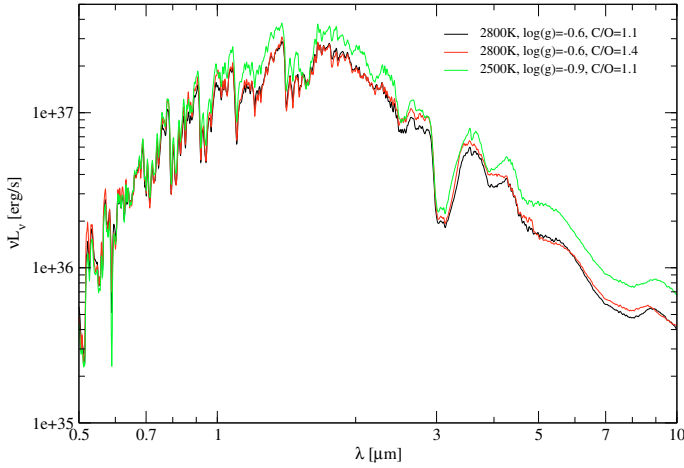
Fig. 3. Three spectra based on COMARCS models with Z/Z_{\odot} = 1.0 , M/M_{\odot} = 1.0 and different values of T_{\text{eff}} , C/O and \log(g) [ \text{cm}/\text{s}^2 ]. The resolution is R = 200 .
