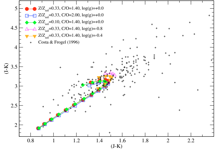
Fig. 18. Two colour diagram (I-K) versus (J-K) for several representative sequences of COMARCS atmospheres characterized by different values of \log(g) [ \text{cm/s}^2 ], Z/Z_{\odot} (denoted as Z/Z_{\text{sol}} in the plot) and C/O. All models have two solar masses. The series start at T_{\text{eff}} = 2600 K and range up to 4000 K for \log(g) [ \text{cm/s}^2 ] = 0.0, up to 3200 K for \log(g) [ \text{cm/s}^2 ] = -0.4 and up to 2900 K for \log(g) [ \text{cm/s}^2 ] = -0.8. The warmest objects correspond to the bluest colours. The data are compared to observations of LMC carbon stars published by Costa & Frogel (1996).
