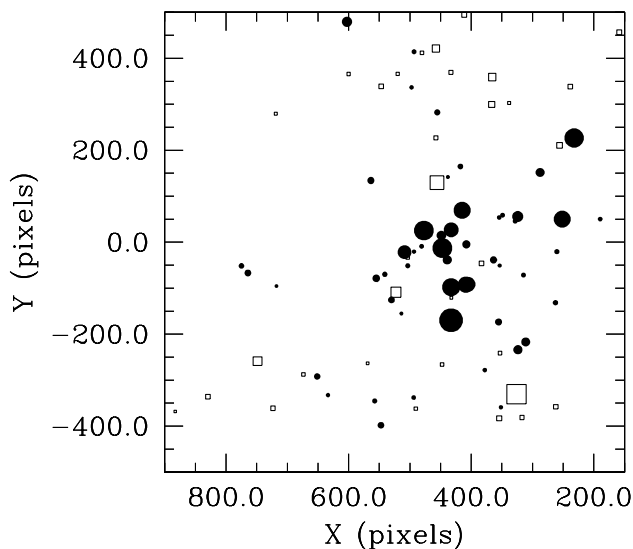
Figure 8. Spatial distribution of candidate members and non-members in the field of Trumpler 15 having UBV photometry. Symbols are as in Fig. 5 and the size of the stars is proportional to their magnitudes.
