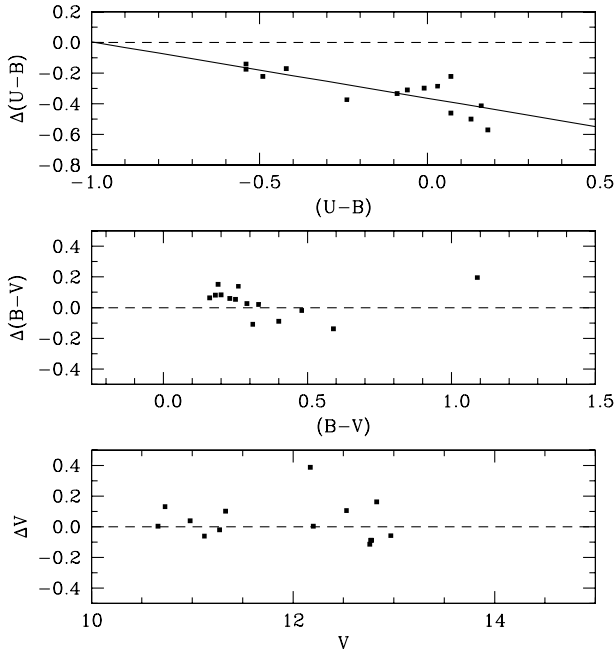
Figure 2. A comparison of our photometry with Thé & Vleeming (1971) study. The comparison is in the sense (this study–Thé & Vleeming).
