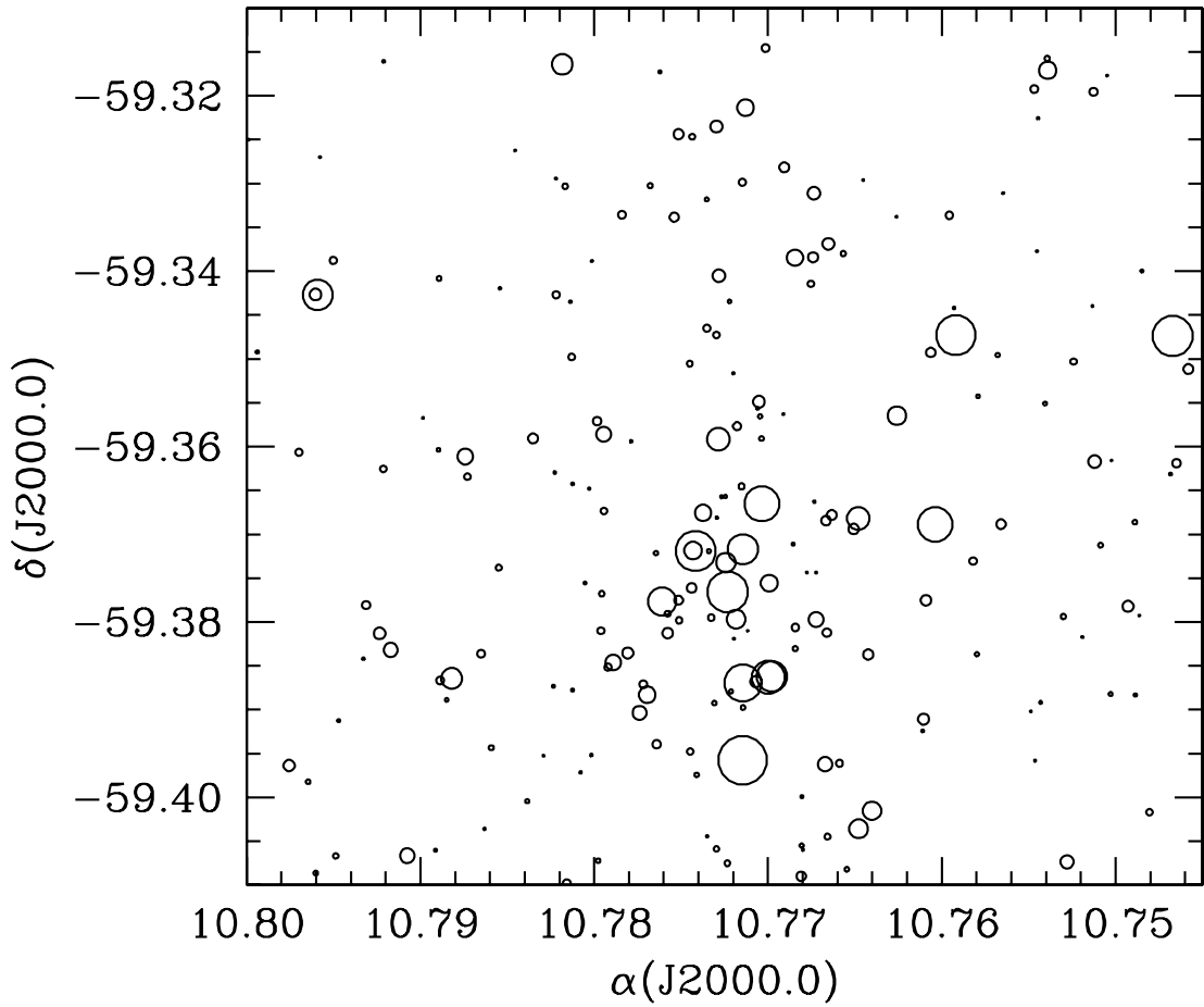
Figure 1. A map of an observed region around Trumpler 15. The size of each star is proportional to its magnitude. North is up, east on the left. The field is about 6 \times 6 arcmin 2 .
