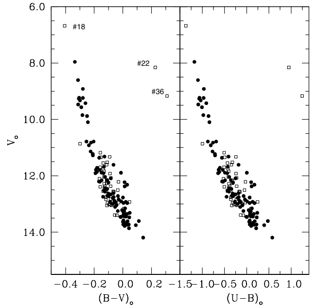
Figure 7. Reddening corrected CMDs for stars in the field of Trumpler 15 having UBV photometry. Symbols are as in Fig. 5. Some interesting stars have been labelled with their Grubissich number.
