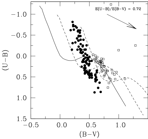
Figure 5. Two-colour diagram for stars in the field of Trumpler 15 having UBV photometry. Filled circles indicate stars having mean reddening E(B - V) = 0.52 \pm 0.07 (rms), open squares stars with larger reddening. The solid line is the empirical ZAMS from Schmidt-Kaler (1982), whereas the dashed lines are the same ZAMS, but shifted by E(B - V) = 0.30 and by E(B - V) = 0.70 , respectively.
