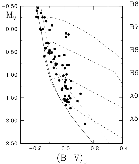
Figure 12. A zoom of the lower part of the reddening corrected CMDs. The solid line is a post-MS isochrone for the age of 6 \times 10^6 yr, the dotted line in the left panel is the same isochrone, but shifted by 0.70 to mimic the locus of unresolved binaries, and the dashed lines are from the bottom to the top pre-MS isochrones for the ages of 2, 3, 5 and 7 \times 10^6 yr.
