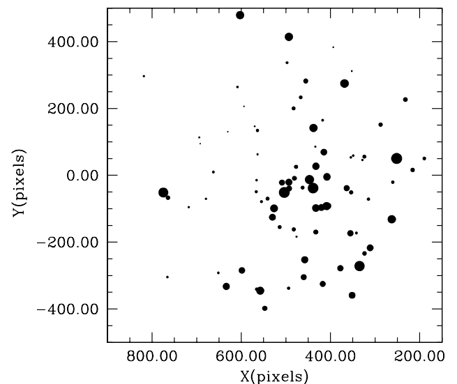
Figure 9. Spatial distribution of colour excesses of the candidate member stars in the field of Trumpler 15. The size of each star is proportional to its colour excess.
