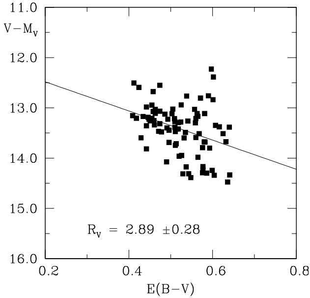
Figure 10. Differential reddening plot for all the MS stars in the studied region. The solid line is a least-squares fit through the data.
