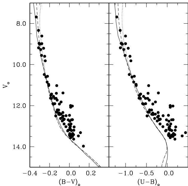
Figure 11. Reddening corrected CMD for the stars members of Trumpler 15. The solid line is the empirical ZAMS form Schmidt-Kaler (1982) Superimposed are post-MS isochrones from Girardi et al. (2000) (dashed and dotted lines). See text for more details.
