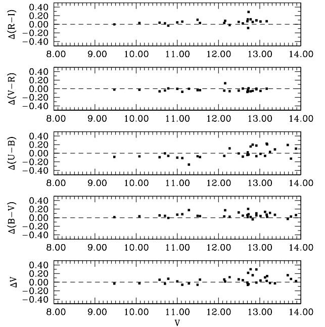
Figure 3. A comparison of our photometry with Feinstein et al (1980) study. The comparison is in the sense (this study–Feinstein et al).
