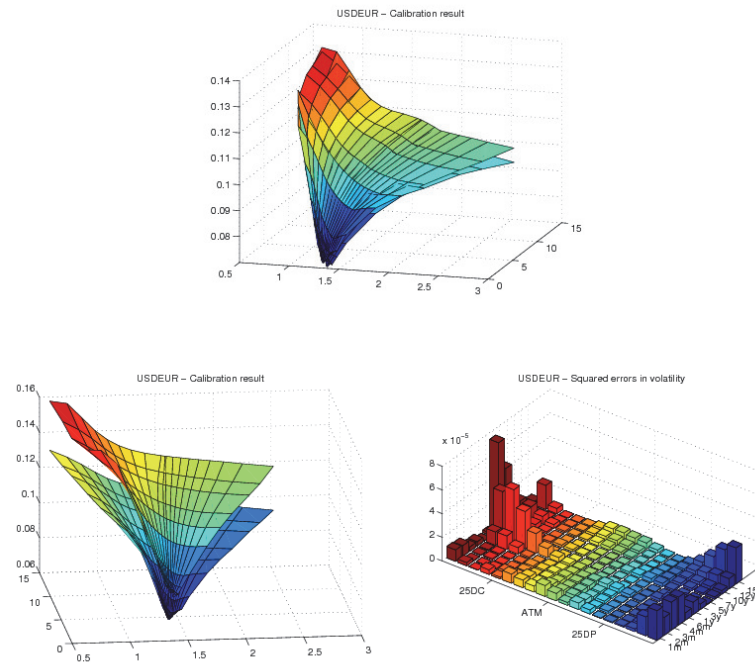
Figure 5. We simultaneously consider a joint calibration of the implied volatility surface of USDEUR and of the two yield curves of USD and EUR. The top figure compares the implied volatility surface to observed market data. As the fit is very good and the two surfaces are almost indistinguishable, in the bottom left figure we shift upwards the model-implied volatility by multiplying each point by 1.1 so as to increase readability. In the bottom right figure we report squared errors in implied volatility for each point of the surface.
