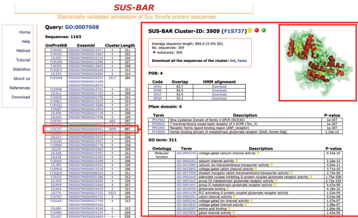
Figure 2. SUS-BAR sequences endowed with statistically validated GO terms corresponding to the sensory perception of smell. The left panel lists all the pig sequences that are retrieved when the database search is done with GO:0007608. In all, 1163 pig sequences in SUS-BAR inherit the same statistically validated GO term by entering clusters where the term is statistically validated by computing its Bonferroni-corrected P -value (19). Characteristics of the cluster (#3909) where one of these 1163 pig protein sequences (F15737, red box in the left) is located are shown in the right panel. Structural alignment of the four PDBs contained in the clusters is done with Mustang (25) and visualized with PyMol ( http://www.pymol.org ). The inset is manually computed for the figure and is not present in the corresponding page of the Web site. Each pig protein sequence in the cluster can be, however, modelled in house after downloading of the corresponding alignment with the templates in the cluster. This is provided with the cluster-specific HMM. See text for further details. Yellow stars indicate that the GO term is statistically validated and endowed with an experimental evidence code. The red dot indicates that the cluster contains SwissProt annotated proteins.
