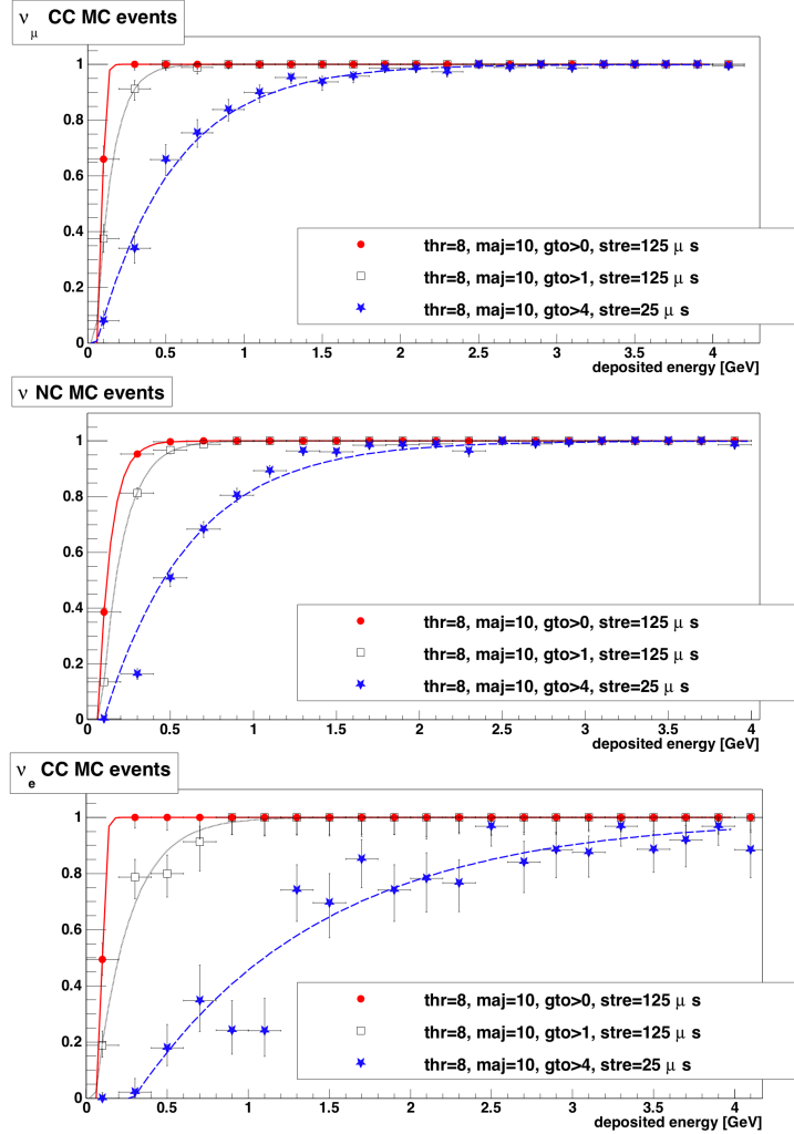
Figure 20. SD CNGS trigger efficiency for \nu_\mu CC (top), \nu NC (center) and \nu_e CC (bottom) MonteCarlo events as a function of the deposited energy, for three parameter configurations. The effective live-time of each SD board has been accounted for in the analysis.
