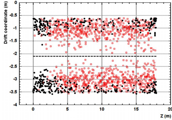
Figure 8. Spatial distribution of cosmic muon tracks in the WEST module as triggered by PMTs (red squares) and below the PMT detection threshold (black circles, see Chapter 4). PMT system inefficiency is mostly localized in the regions where PMTs were switched off.
