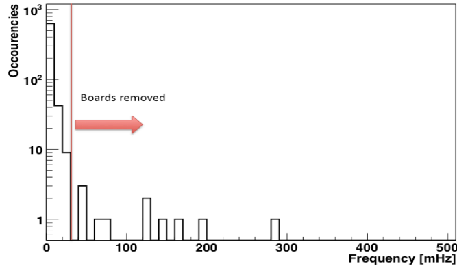
Figure 12. Distribution of the single GTO detection rate for all the ICARUS T600 boards. The bulk of the distribution is below 30 mHz; the few SD chips exceeding this limit have been excluded from the analysis.
