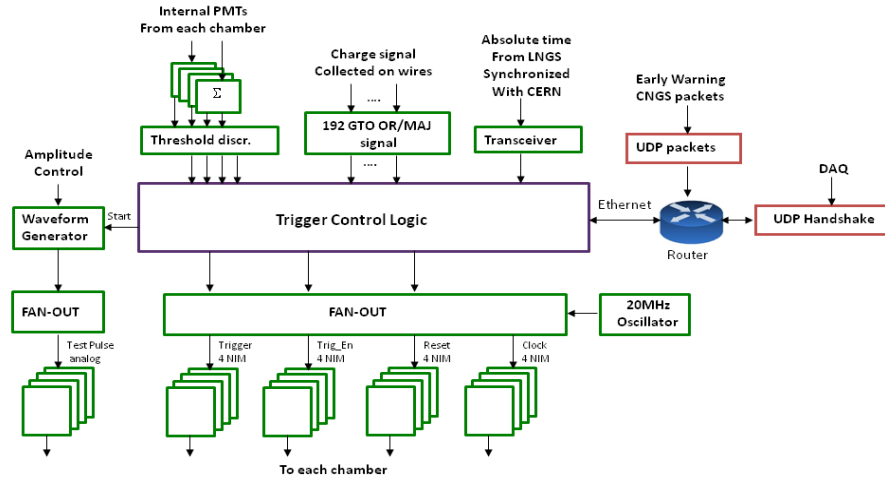
Figure 14. Block diagram of the ICARUS T600 Trigger Manager.
