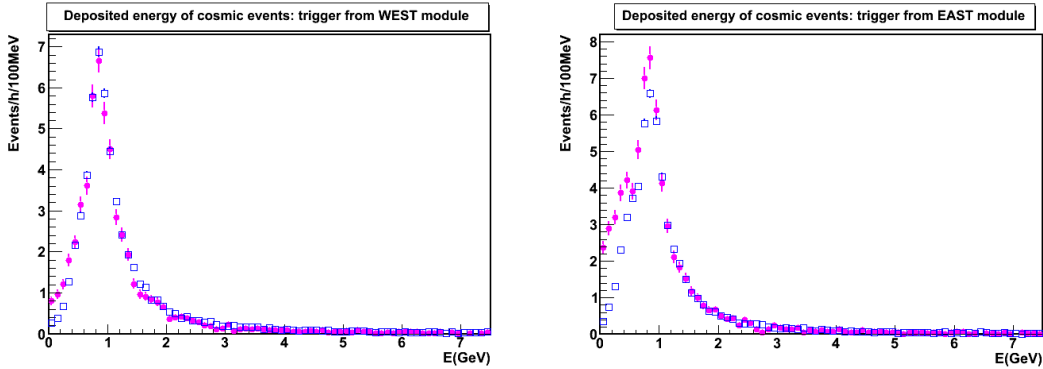
Figure 23. Comparison between the differential cosmic ray spectra in the WEST (left) and EAST (right) modules collected in July 2011 (blue open squares) and in March 2012 (pink full circles), after the PMTs improvements carried out from December 2011 to March 2012.
