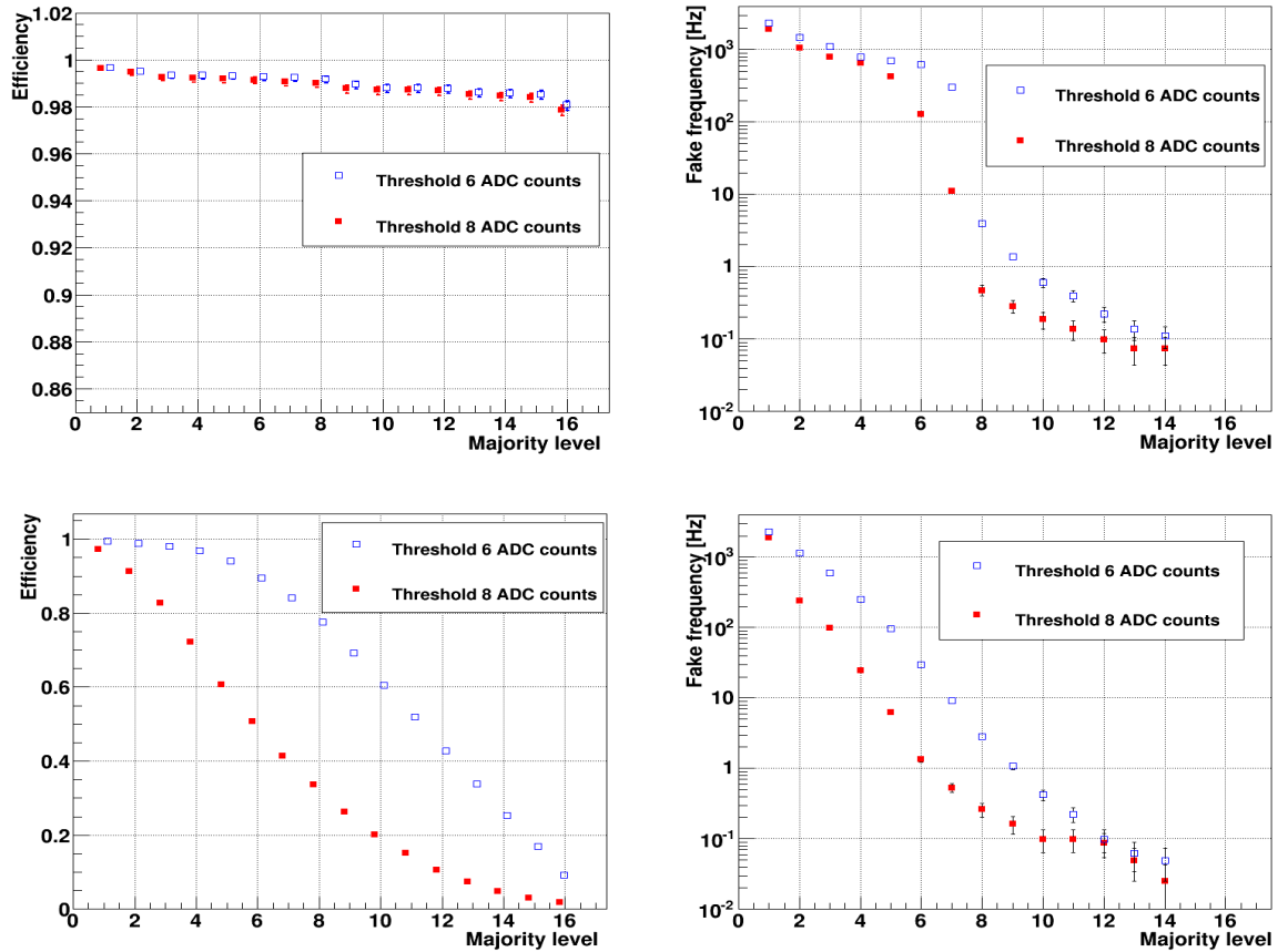
Figure 13. Top. Single GTO detection efficiency for vertical muon tracks (left) and corresponding rate of fake triggers (right) in Collection view as a function of the majority level for two different threshold values. The drop of the fake rate around MAJ = 7 is due to the exclusion of the noisy boards. Bottom. The corresponding GTO detection efficiency and fake rate as measured in Induction2 view. No fake triggers have been recorded for majority MAJ > 14 in both Collection and Induction2 views.
