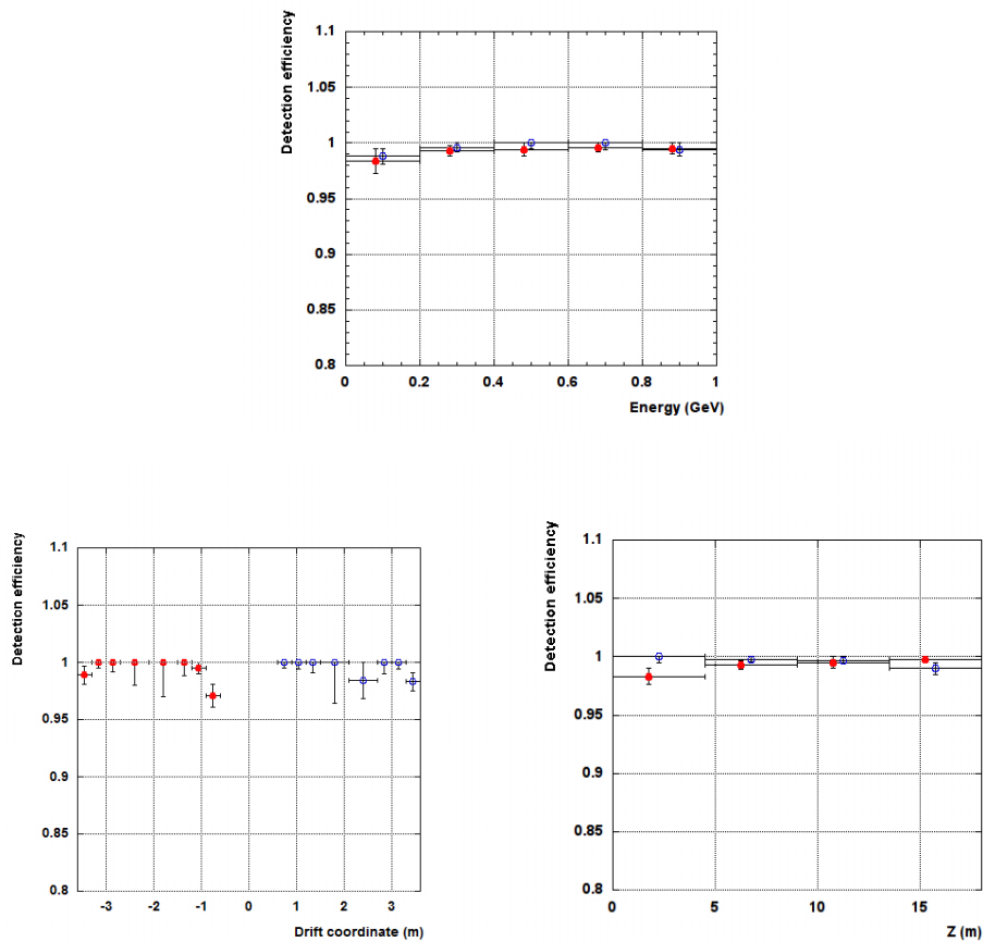
Figure 17. Top: Efficiency of the OR of PMT sum signals in the two TPCs of WEST (red circles) and EAST (blue circles) modules, as a function of deposited energy for cosmic ray muons. The associated systematic uncertainty ranges from 3 (1) % in the lowest energy bin for the WEST (EAST) module down to a negligible level in the highest energy bin for both modules. Bottom: detection efficiency as a function
