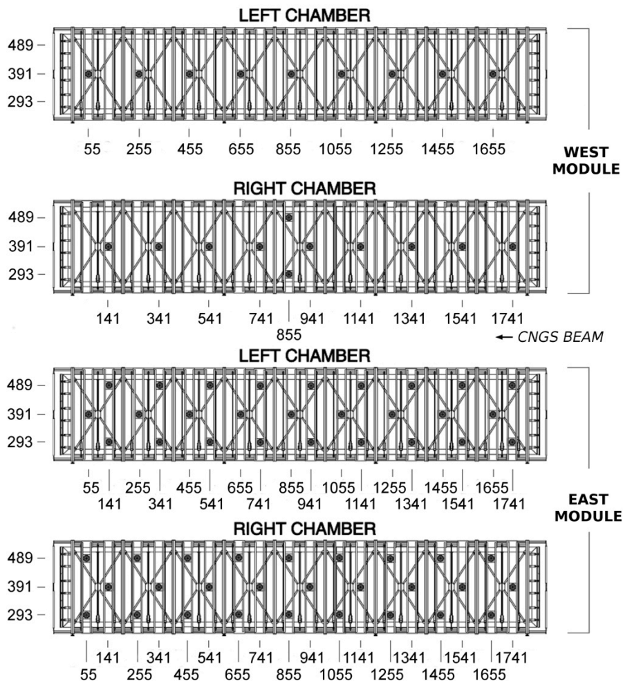
Figure 2. PMT's deployment in the two ICARUS T600 cryostats. PMT coordinates in cm are referred to a reference frame in Hall B whose origin is set at the ground floor (vertical axis, x), at the center of the two modules (drift coordinate, y) and at the downstream end of the wire chambers for the longitudinal direction (z) along the CNGS beam line.
