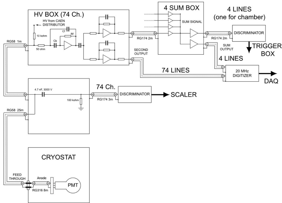
Figure 3. PMT electronics layout.
