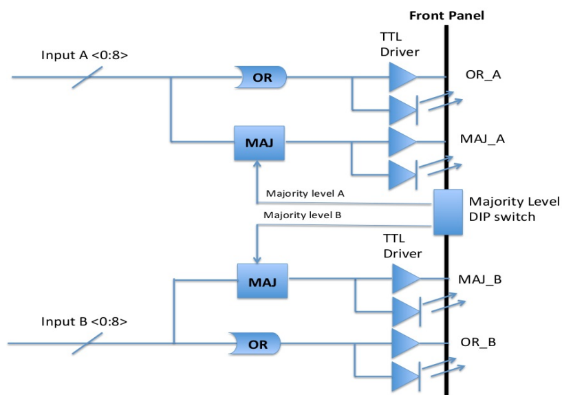
Figure 11. Block diagram of the GTO OR/MAJ board.
