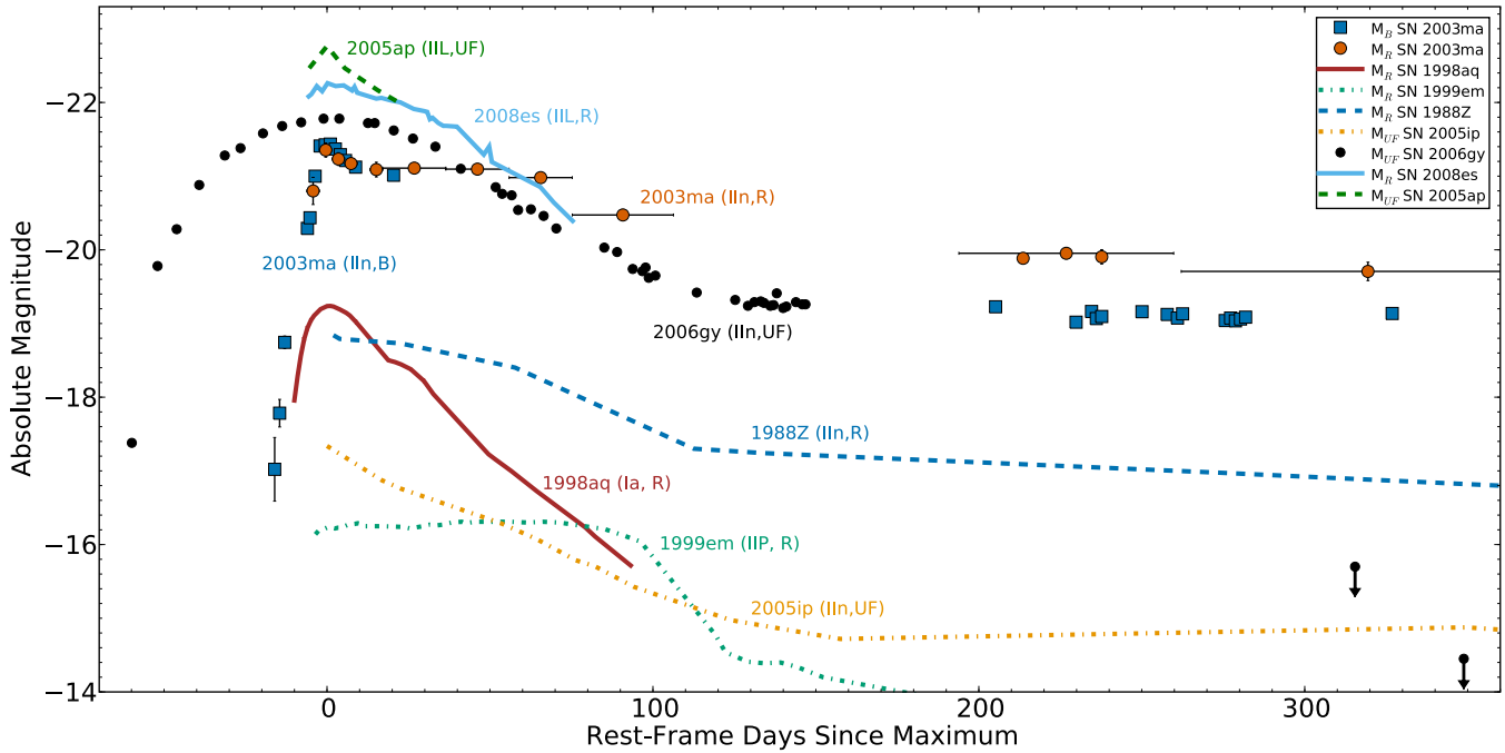
Figure 9. Light curve of SN 2003ma (DM = 40.86 mag, z = 0.289 ) in absolute, rest-frame B - and R -band magnitudes in comparison to SN IIn 1988Z (DM = 34.77 mag; Aretxaga et al. 1999), SN IIn 2005ip (DM = 32.36 mag; Smith et al. 2009b), the extremely luminous SN IIn 2006gy (DM = 34.32 mag; Smith et al. 2007b; Agnoletto et al. 2009), SN IIL 2008es (DM = 40.08 mag, z = 0.21 ; Miller et al. 2009; Gezari et al. 2009a), and SN IIL 2005ap (DM = 40.81 mag, z = 0.283 ; Quimby et al. 2007), SN Ia 1998aq (DM = 31.696; Riess et al. 2005), and SN IIP 1999em (DM = 29.569 mag; Leonard et al. 2002) in rest-frame days since maximum. The times of maxima for SNe 1998aq, 1999em, 2006gy, 2008es, and 2005ap are well constrained, but for SNe 1988Z and 2005ip there are no upper limits before the date of discovery, and so we assume that the date of discovery is the peak date. The light curves are in rest-frame B , R , or R -like unfiltered ( UF ) magnitudes. 32 We do not apply any K -correction to the SNe with distances \lesssim 100 Mpc (SNe 1998aq, 1988Z, 1999em, 2005ip, and 2006gy). We convert the light curve of SN 2008es from observed i band to rest-frame R band by applying a K -correction of -0.043 mag. We convert the light curve of SN 2005ap from unfiltered magnitudes to rest-frame R band by applying a K -correction of 0.054 mag, assuming that the observed magnitudes are in R band. We apply extinction corrections of 0.036 , 0.24 , 0.126 , and 1.78 mag to the light curves of SNe 1998aq, 1999em, 2006gy, and 2005ip, respectively. The published light curves of SNe 1988Z, 2008es, and 2005ap are already extinction corrected. The observed VR and I -band measurements of SN 2003ma are extinction corrected by 0.66 and 1.01 mag, respectively, and then converted into rest-frame magnitudes in B and R bands with K -corrections of -0.63 and -0.51 mag, respectively. All K -corrections are calculated assuming a solar spectrum.
