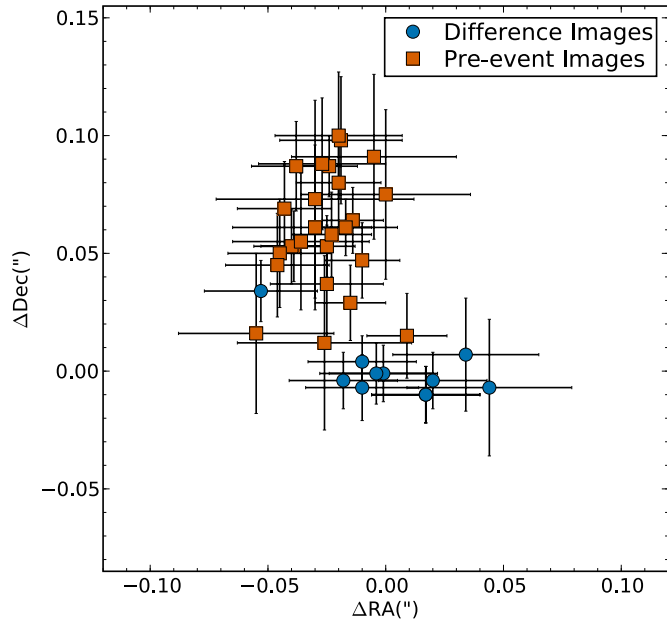
Figure 2. Centroids of the sources at/near the position of SN 2003ma from multiple images. The red squares indicate the centroids of detections in the pre-event ( \text{MJD} \leq 52965 ) SuperMACHO images, while the blue circles indicate the high S/N centroids of SN 2003ma in the SuperMACHO difference images during 52985 \leq \text{MJD} \leq 53020 . SN 2003ma is offset from the template source by 0.064 \pm 0.012 arcsec, indicating that it is at a projected distance of d \approx 460 \pm 85 pc from the host.
