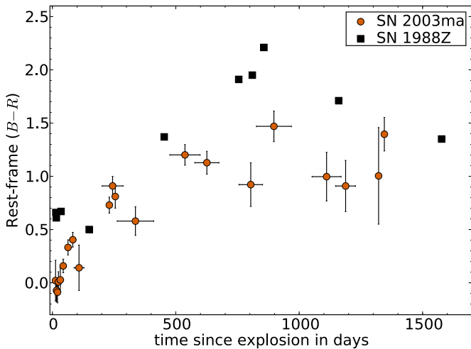
Figure 11. Rest-frame B - R colors of SN 2003ma in comparison to SN 1988Z in days since the estimated time of explosion t_0 . The time of explosion of SN 1988Z is assumed to be 12 days before discovery. The time axis is in the rest frame. Both SNe show an increase in B - R color until \sim 1000 days, after which the B - R color plateaus.
