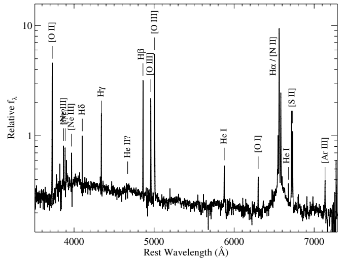
Figure 6. Optical spectrum of SN 2003ma from 2008 ( t = 1423 days). Narrow emission lines are marked. The continuum is likely dominated by the host galaxy, while the broad H \alpha and potential He \pi \lambda 4686 lines are from SN 2003ma.
