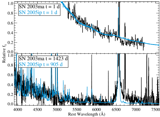
Figure 7. Optical spectra of SN 2003ma compared with those of SN 2005ip. Phases are given in rest-frame days since maximum light. Top: galaxy-template subtracted maximum-light spectrum of SN 2003ma (black) and maximum-light spectrum of SN 2005ip (blue). An additional E(B - V) = 0.9 mag of internal extinction was applied to SN 2005ip to match the continuum shape of SN 2003ma. Bottom: the 1423 day (4 year; black) and 905 day (2.5 year; blue) spectra of SN 2003ma and SN 2005ip, respectively. A template galaxy spectrum has been added to the SN 2005ip spectrum to match the continuum shape of the SN 2003ma spectrum.
