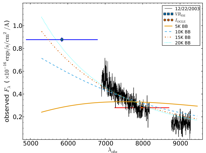
Figure 13. Spectrum of SN 2003ma (black line) from 2003 December 22 ( \sim 3 days after peak) with galaxy contamination subtracted as discussed in Section 3.1 and dereddened. The galaxy H \alpha line does not fully subtract. Therefore, the spectrum in the rest-frame wavelength range 6350–6800 Å is not reliable and we do not use it in the analysis. Overplotted are the dereddened observed fluxes derived from the VR_{\text{SM}} (blue squares) and I_{\text{OGLE}} (red diamonds) photometry. The horizontal error bars indicate the width of the filters. The solid orange line, dashed sky blue line, dot-dashed purple line, and dotted cyan line indicate blackbody fits of 5000, 10,000, 15,000, and 20,000 K to the spectrum and photometry, respectively.
