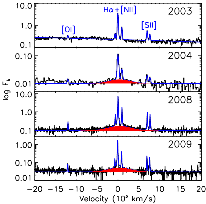
Figure 8. Narrow [O I] \lambda 6300 , H\alpha , [N II] \lambda\lambda 6548, 6583 , and [S II] \lambda\lambda 6716, 6731 emission lines fitted with Voigt profiles with a width equal to the [N II] \lambda 6583 line in each spectrum, respectively, are shown with a blue line. In 2003 the continuum is fitted with a quadratic function, and in 2004, 2008, and 2009 the continuum is fitted with a constant value. An additional broad Gaussian component that is needed to fit the H\alpha line in 2004, 2008, and 2009 is shown in red. In 2004 the [N II] \lambda 6548 line is not detected above the noise, and is weaker than expected for a line ratio of 3:1 for [N II] \lambda 6583/\lambda 6548 .
