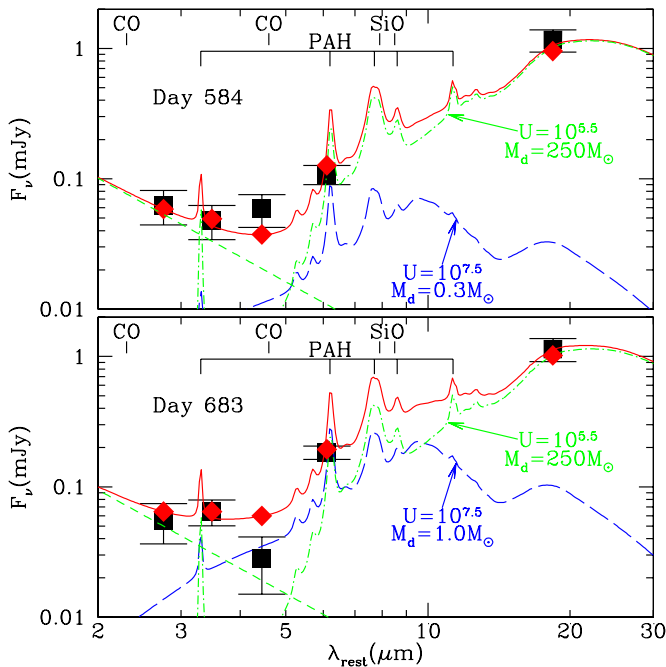
Figure 15. Spitzer IRAC (3.6, 4.5, 6.0, and 8.0 \mu\text{m} ) and MIPS (24 \mu\text{m} ) photometry vs. rest wavelength, for 584 and 683 days after maximum. The solid curves show models which include hot dust, warm dust (see the text), and a stellar component with a Rayleigh–Jeans spectrum. Filled diamonds are the model convolved with the IRAC and MIPS response functions. The photometry is consistent with the observed emission consisting of steady emission from warm dust in the galaxy, plus a time-variable IR echo produced by hot dust. (A color version of this figure is available in the online journal.)
