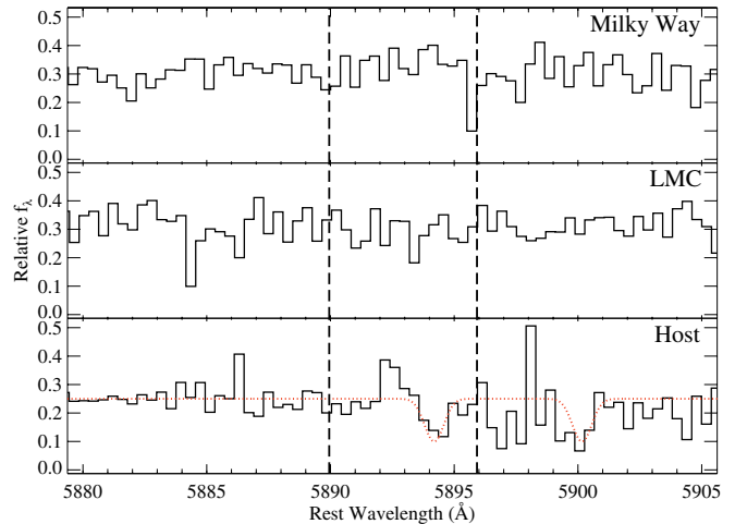
Figure 12. Optical spectrum of the 1423 day spectrum of SN 2003ma near the rest wavelength of the Na D doublet for the Milky Way (top), LMC (middle), and host galaxy (bottom), respectively. The vertical dashed lines indicated the wavelengths of the Na D lines. We detect no Na D absorption in the Milky Way or LMC to a equivalent width limit of \sim 0.4 Å. There is the possibility of Na D absorption in the host galaxy with a redshifted velocity of 200 km s -1 relative to the host galaxy with an equivalent width of 0.5 Å. This possibility is represented by the red dashed lines.
