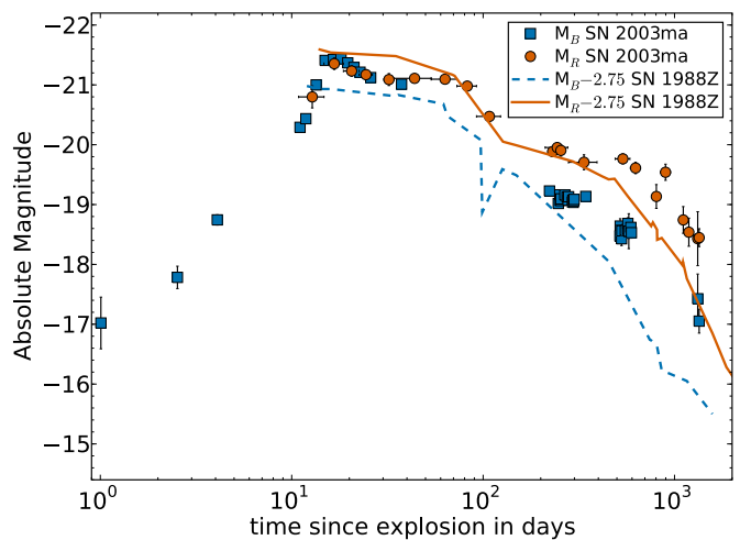
Figure 10. Light curve of SN 2003ma in absolute magnitudes in comparison to SN 1988Z in days since explosion, on a log scale. The time axis is in the rest frame. Offsets have been added to the SN 1988Z absolute magnitudes in order to compare the shape of the light curves. Since the time of explosion is not well constrained for SN 1988Z, we shift the light curves by 12 days to match the bend in the I -band light curve of SN 2003ma seen after 100 days.
