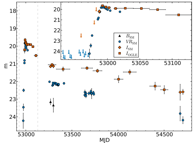
Figure 4. Optical light curves of SN 2003ma. The black triangles, blue circles, orange diamonds, and orange squares show the apparent magnitudes in the natural system of B_{SM} , VR_{SM} , I_{SM} , and IOGLE , respectively. Because of the low S/N of a single detection, we average IOGLE (orange squares), with the range of epochs used to calculate this average indicated by the error bars along the time axis. The inset shows the light curve during peak from 52928 \leq \text{MJD} \leq 53130 , and the 3\sigma brightness upper limits.
