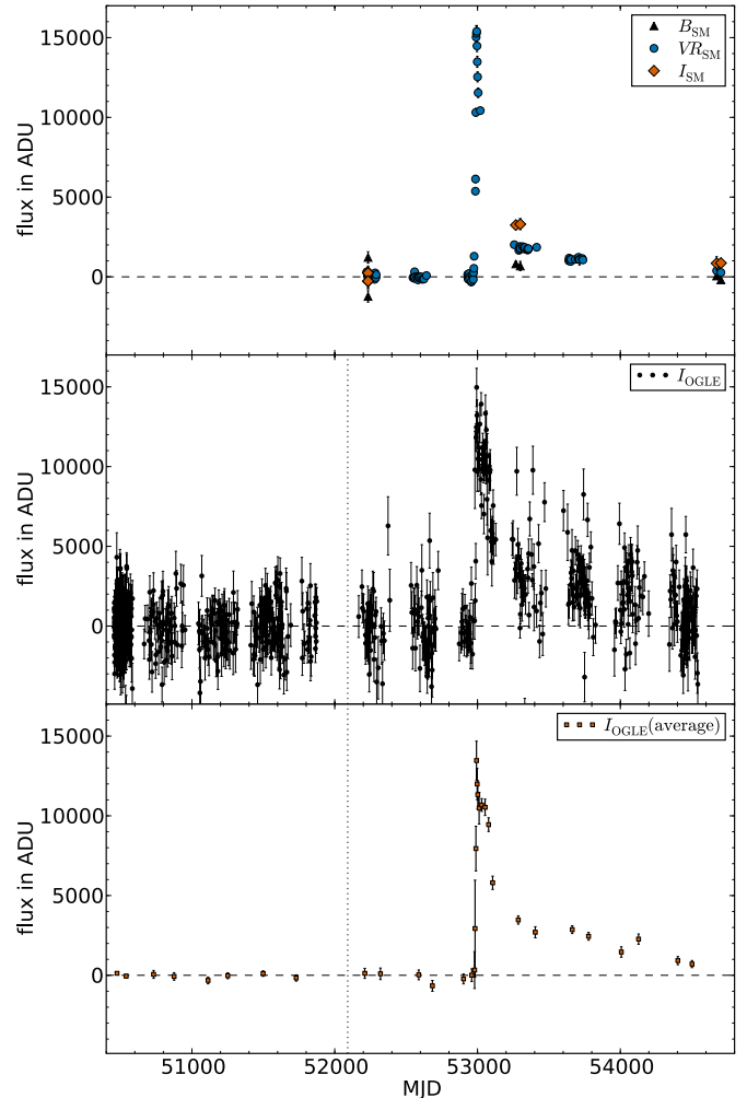
Figure 3. Difference image light curves of SN 2003ma. Top: black triangles, blue circles, and orange diamonds show the SuperMACHO difference flux light curves in B_{\text{SM}} , VR_{\text{SM}} , and I_{\text{SM}} , respectively, from 2001 November 11 to 2008 August 25. Middle: small black circles indicate the I_{\text{OGLE}} difference flux light curves. Bottom: because of the low S/N of a single detection, we average the data (orange squares). The horizontal dashed lines indicate zero flux. The vertical dotted line indicates the transition between OGLE-II and OGLE-III measurements.
