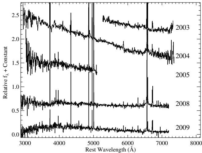
Figure 5. Optical spectra of SN 2003ma. The spectra are denoted by the year in which they were obtained. The spectra in years 2003, 2004, 2005, and 2008 correspond to rest-frame phases of 1, 279, 905, and 1423 days relative to B maximum, respectively. There is significant galaxy contamination in all spectra, likely dominating the spectrum at later phases. Since the 2004 spectrum was not obtained at the parallactic angle, its spectral shape is likely incorrect.
