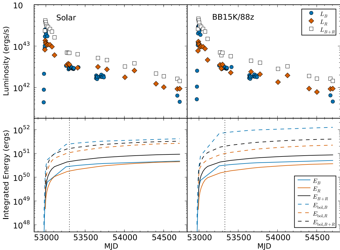
Figure 14. Top left: the luminosities in the rest-frame B , R , and combined B + R passbands using the solar SED for the determination of the K -correction (solar model). Top right: same luminosities, but using a 15,000 K blackbody SED for the K -correction during peak, and SEDs from SN 1988Z for the K -corrections during the plateau phase (BB15K/88Z model). Bottom left and right: the integrated emitted energy in the B , R , and combined B + R passbands using the solar and BB15K/88Z model, respectively, in solid lines. The dashed lines show the integrated bolometric energy for the two models. See Section 4.5 for a discussion.
