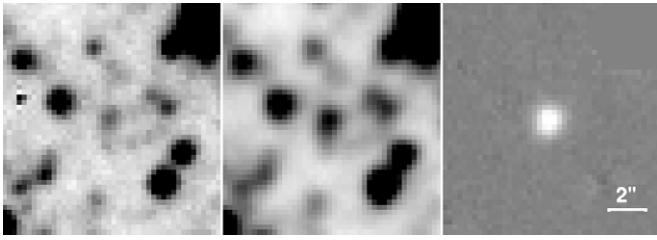
Figure 1. SuperMACHO images of the region around SN 2003ma. Left: template image from 2001 November 20 (pre-event). Middle: search image from 2003 December 17, showing a detection of SN 2003ma at the center of the image. Right: difference image (center minus left with an inverted color scale) clearly showing the detection of SN 2003ma. The white line in the lower right corner indicates 2'' . North is up and east is left.
