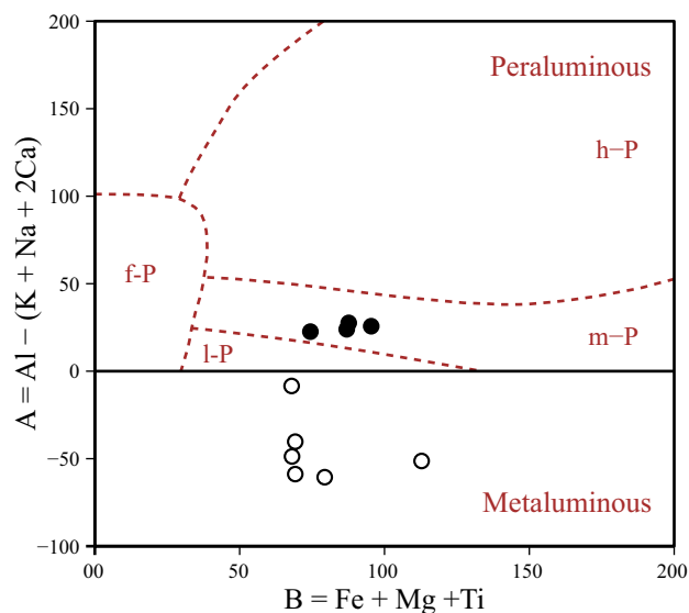
Figure 7. A-B plot (modified by Villaseca et al. , 1998), with A = [Al - (K + Na + 2Ca)] and B = Fe + Mg + Ti (gram-atoms \times 10^3 of each element in 100 g of materia). Note that all the Sierra de Catorce samples (black dots) are moderately peraluminous, while the Sierra El Fraile samples (open dots) from Pinto-Linares et al. (2008) are metaluminous. f-P: highly felsic peraluminous; l-P: low peraluminous; m-P: moderately peraluminous; h-P: highly peraluminous.
