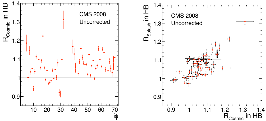
Figure 7. Left: Ratio, for cosmic ray muons, of the average signal amplitudes in the two halves (+z and -z) of HB, as a function of the \phi sector index, i\phi , after correcting the average signal for the muon path length and normalizing to the thickness of HB at \eta = 0 . Right: Correlation between cosmic ray muon and splash muon signals, for the ratio of the average signal in the two halves of HB. The splash muon signals were corrected for the asymmetry in the muon flux by comparing the events from the beam arriving from the +z side and the -z side.
