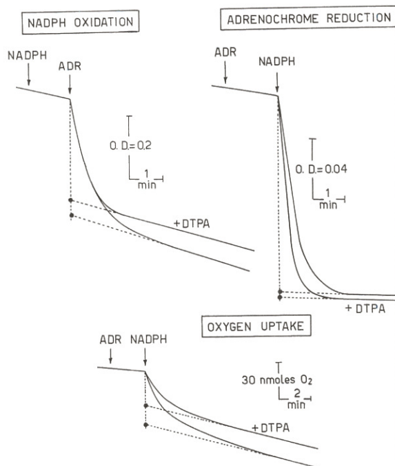
FIGURE 1 Simultaneous measurement of NADPH oxidation, adrenochrome reduction and oxygen uptake during the action of DT-diaphorase on adrenochrome. The reaction mixture was formed by 50 mM Na-K phosphate buffer (pH 7.4), 3 mg/ml protein, 0.2 mM NADPH and 50 \mu M adrenochrome; when indicated, also 1 mM DTPA was added.
