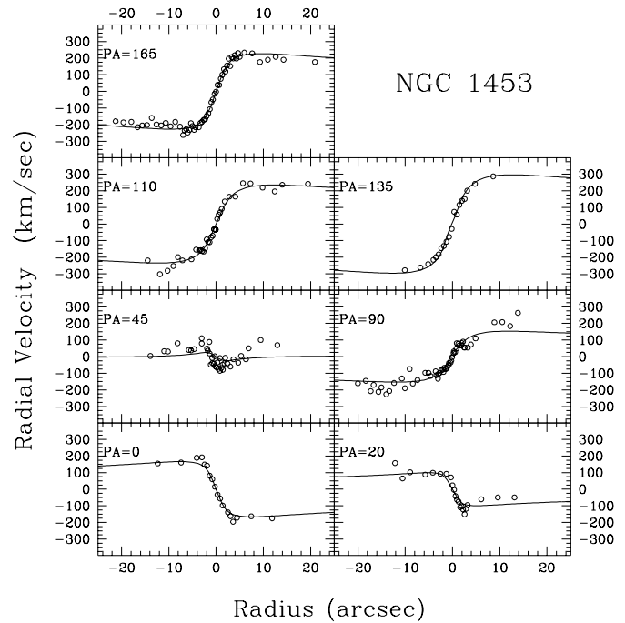
Fig. 1. Observed (open dots) and model (full line) radial velocities curves for NGC 1453.
