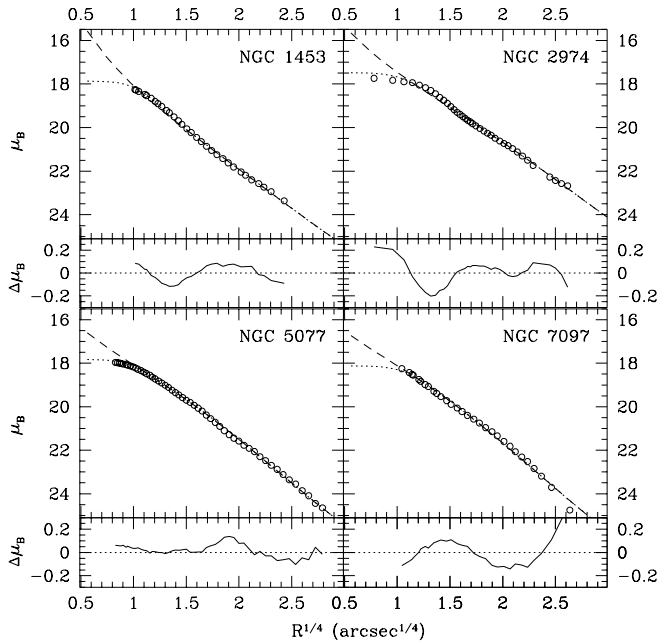
Fig. 2. Modeling the surface brightness profile of the four galaxies studied. In the upper panels the observed (open dots) and model surface brightness profile along the major axis of the objects are plotted. The dashed and dotted lines represents the model profile before and after the seeing convolution respectively. In the lower panels the full line represents the residuals \Delta\mu = (\mu_{\text{observed}} - \mu_{\text{convolved model}}) .
