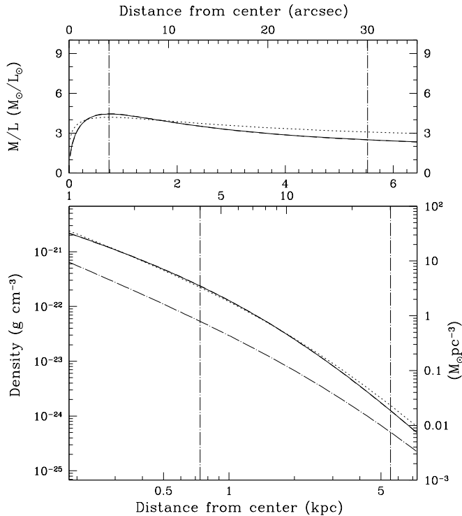
Fig. 5. As Fig. 3 for NGC 2974. The 68% confidence region is bounded by the highest M/L model (dotted line) and by the best model (full line) that, in this case, represents also the lowest M/L model.
