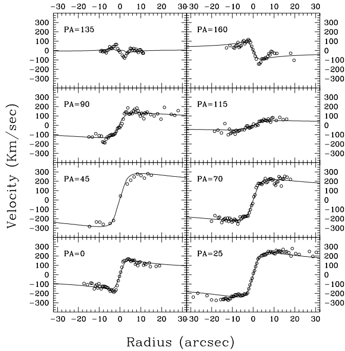
Fig. 4. Observed (open dots) and model (full line) radial velocities curves for NGC 2974.
