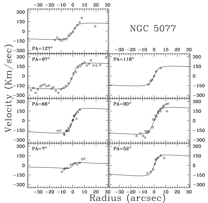
Fig. 6. Observed (open dots) and model (full line) radial velocities curves for NGC 5077.
