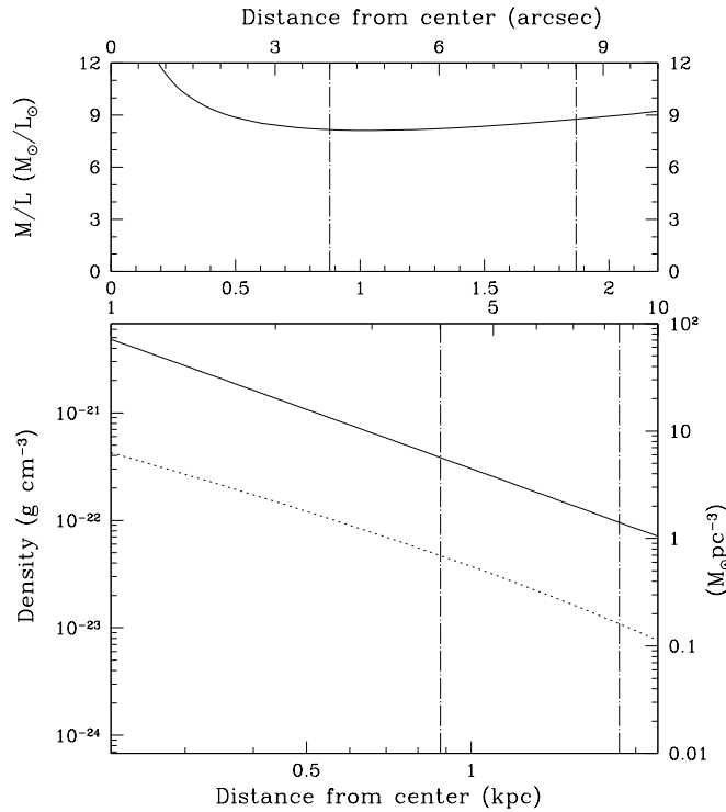
Fig. 9. As Fig. 3 for NGC 7097. Only the best fit model is plotted.
