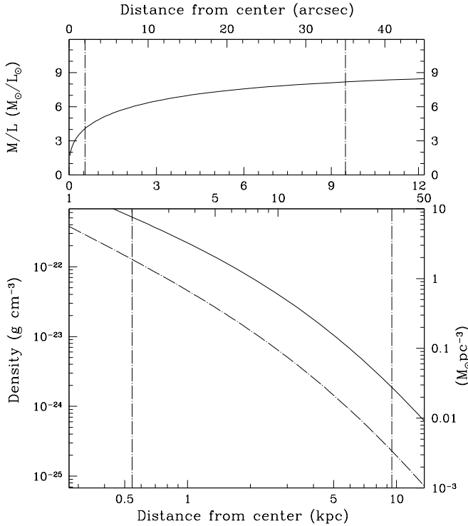
Fig. 7. As Fig. 3 for NGC 5077. Only the best fit model is plotted.
