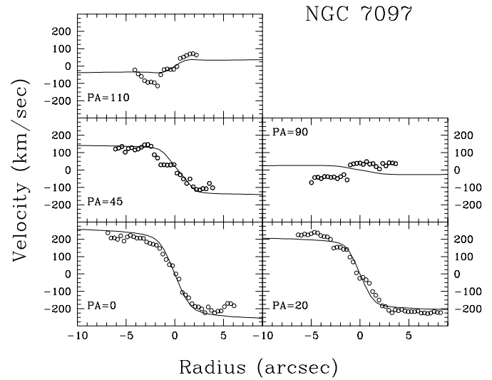
Fig. 8. Observed (open dots) and model (full line) radial velocities curves for NGC 7097.
