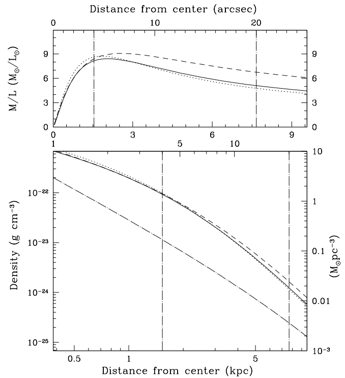
Fig. 3. NGC 1453. Lower panel: mass and light (long dashed line) density profiles for the triaxial model listed in Table 2; the different lines represents the best fit kinematical model (full line) and the two models with the highest and lowest M/L values at large r at the edge of the 68% confidence region (dotted and dashed lines). The radial distance is measured along the intermediate axis. Upper panel: local M/L_B ratio given by the ratio of the profiles of the lower panel. The vertical lines in both the lower and upper panels define the spatial region within which the M/L profile is valid. The inner limit is due to the seeing while the outer limit represents the outermost last available kinematical measurement.
