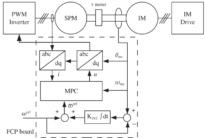
Fig. 7. Schematic of the laboratory test bench.
