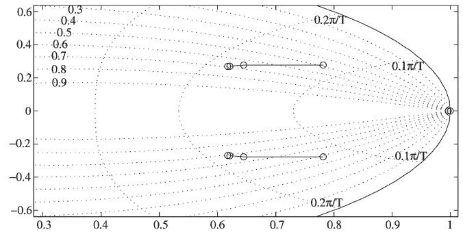
Fig. 6. Pole map for differential input voltage weight \gamma_u = 0.08, 0.8, and 8 .
