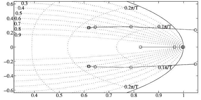
Fig. 5. Pole map for quadrature current weight \gamma_{i_q} = 0, 0.1, 1, and 10 .
