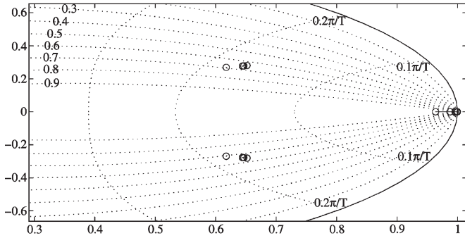
Fig. 4. Pole map for speed error weight \gamma_{\omega_{me}} = 3, 10, 30, 100, and 300 .
