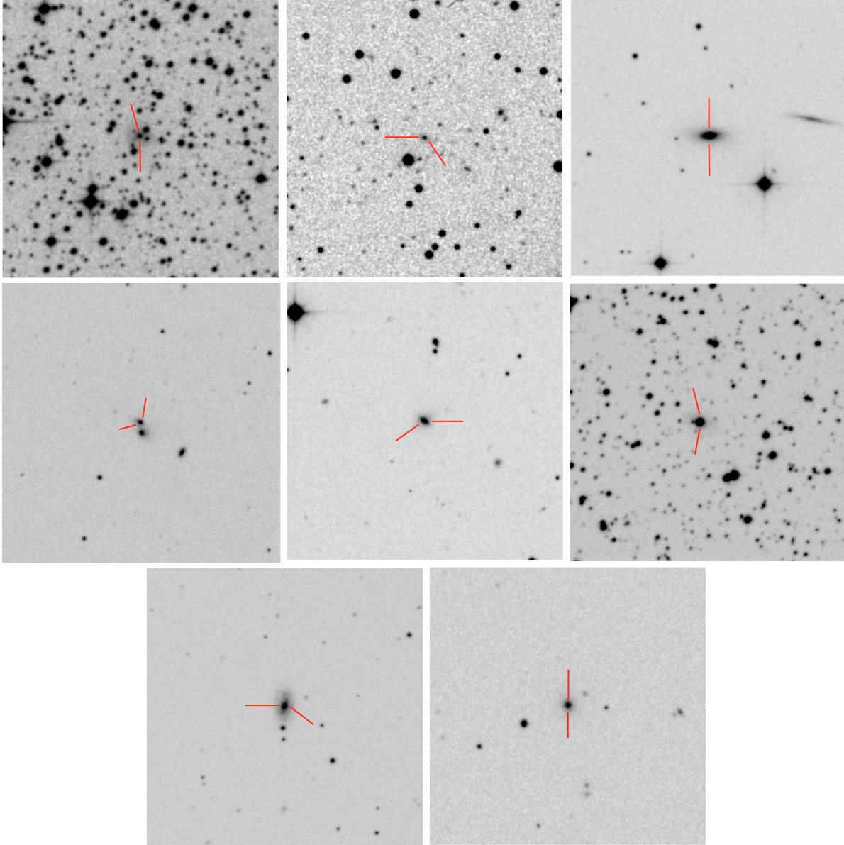
Fig. 2. As Fig. 1, for the fields of Swift J0743.0–2543, Swift J0811.5+0937, Swift J0902.0+6002, Swift J0904.3+5538, Swift J 0911.2+4533, Swift J0917.2–6221, Swift J0923.7+2255 and Swift J1049.4+2258. The optical counterparts of the Swift sources are indicated with tick marks. Field sizes are 5' \times 5' and are extracted from the DSS-II-Red survey. In all cases, North is up and East to the left.
