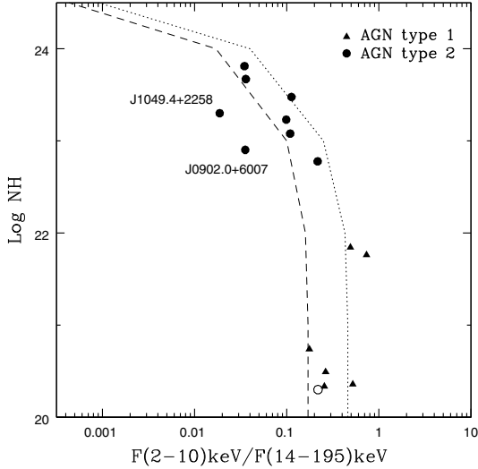
Fig. 7. F_{2-10 \text{ keV}}/F_{14-195 \text{ keV}} flux ratio of our sample. Lines correspond to expected values for an absorbed power law with photon index 1.5 (dot) and 1.9 (dash). The open circle shows the position of Swift J0501.9-3239, the Seyfert 2 without local absorption.
