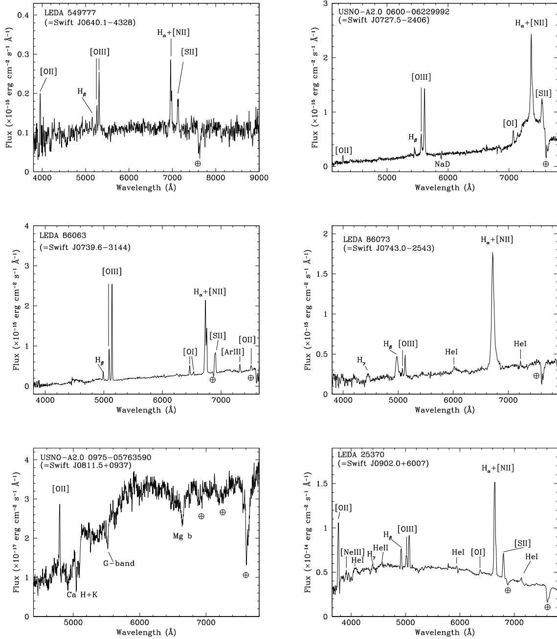
Fig. 4. Spectra (not corrected for the intervening Galactic absorption) of the optical counterpart of Swift J0640.1–4328, Swift J0727.5–2406, Swift J0739.6–3144, Swift J0743.0–2543 and Swift J0811.5+0937, Swift J0902.0+6007.
