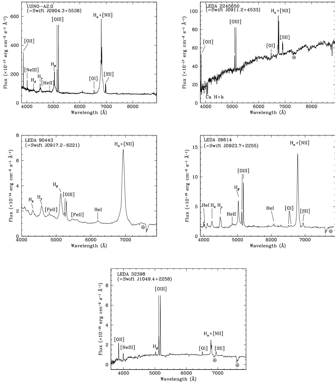
Fig. 5. Spectra (not corrected for the intervening Galactic absorption) of the optical counterpart of Swift J0904.3+5538, Swift J0911.2+4533, Swift J0917.2-6221 and Swift J0923.7+2255, Swift J1049.4+2258.
