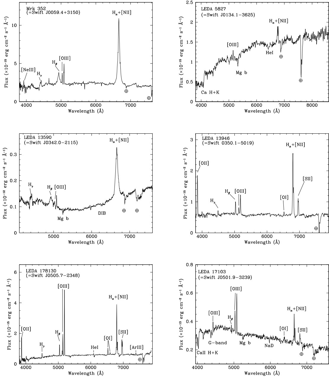
Fig. 3. Spectra (not corrected for the intervening Galactic absorption) of the optical counterpart of Swift J0059.4+3150, Swift J0134.1-3625, Swift J0342.0-2115, Swift J0350.1-5019, Swift J0505.7-2348 and Swift J0501.9-3239.
