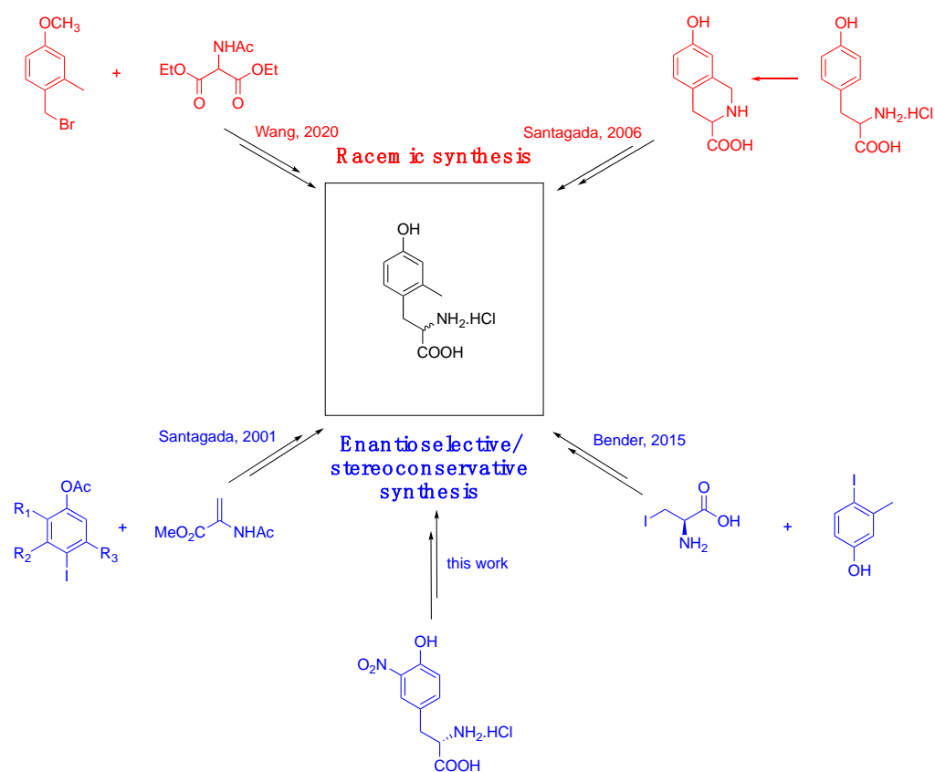
Figure 1. Brief comparison between previous Mmt syntheses [24,26–28] and this work.
