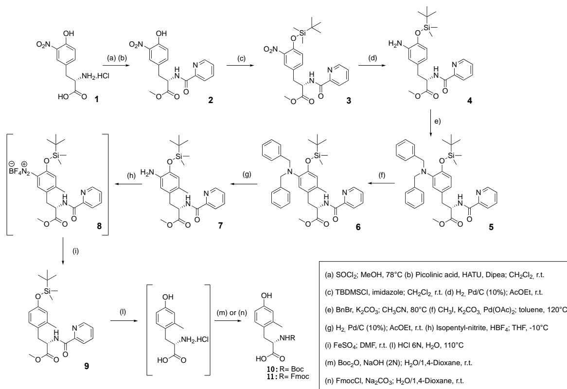
Figure 3. Traceless bulky regioselective synthesis of Mmt via Pd-catalyzed \text{C}(\text{sp}^2)\text{-H} activation.
