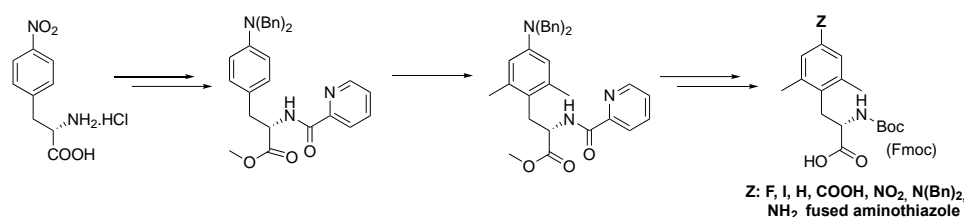
Figure 2. Dmt synthesis via Pd-catalyzed \text{C}(\text{sp}^2)\text{-H} , Trapella, and Poli pathway.
