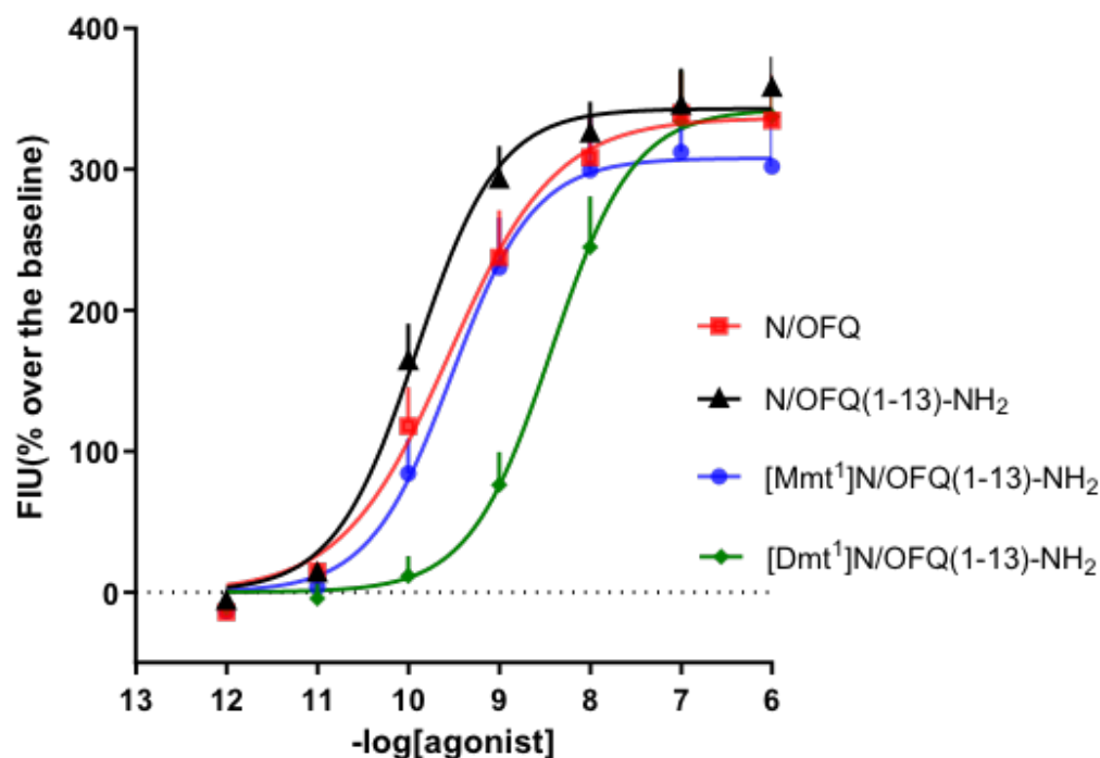
Figure 5. Calcium mobilization assay in CHO cells stably expressing the NOP receptor and the G_{\alpha_{qi5}} chimeric G protein. Concentration–response curves to N/OFQ, N/OFQ (1-13)-NH 2 , [Mmt 1 ] N/OFQ (1-13)-NH 2 , and [Dmt 1 ] N/OFQ (1-13)-NH 2 . Data are mean \pm SEM of at least 6 separate experiments made in duplicate.
