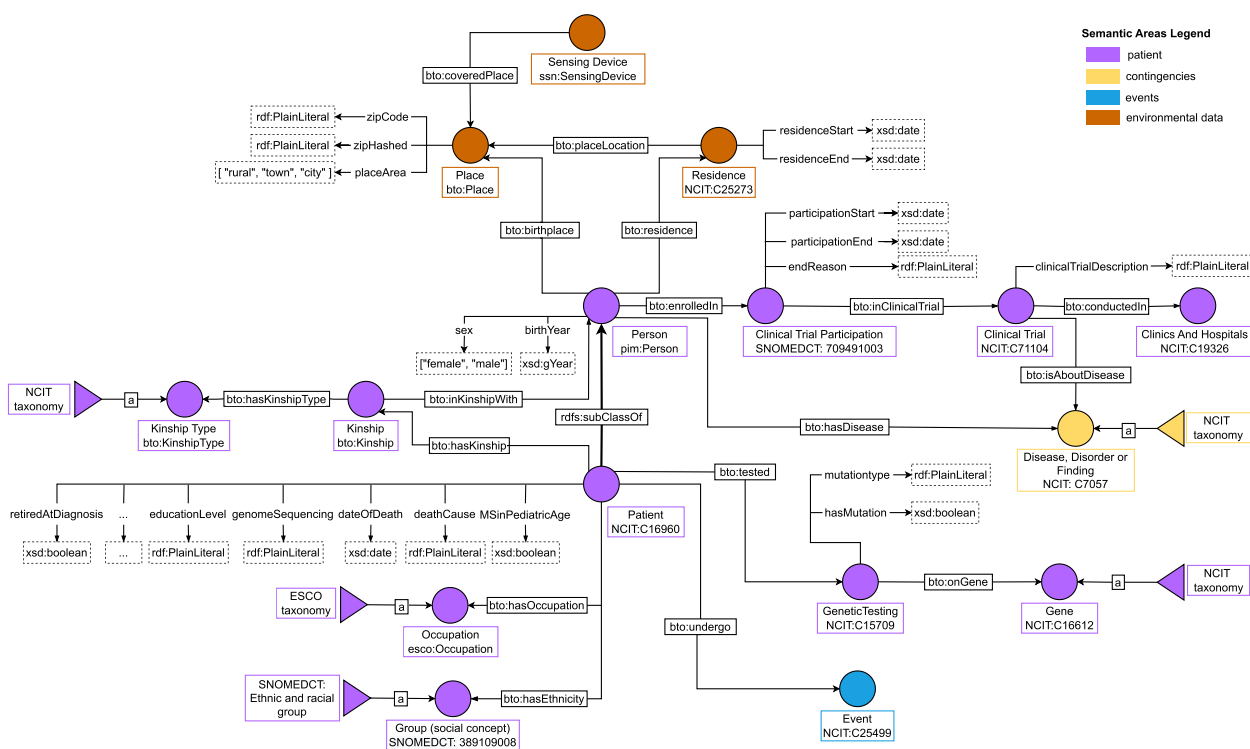
Fig. 3 Patient semantic area, identified by the color purple. In particular, yellow specifies the “Contingencies” areas classes, azure defines events and brown recognizes classes related to environmental information. Patient is a subclass of the class Person from Friend-Of-A-Friend (FOAF) ontology. We directly connect to patient data about genetic mutations, occupation, family history, and residence place. The latter is useful to link environmental information to each patient, which is modeled by importing the “Global City Indicator Environment Ontology” [33]. See Table 9 for the legend
