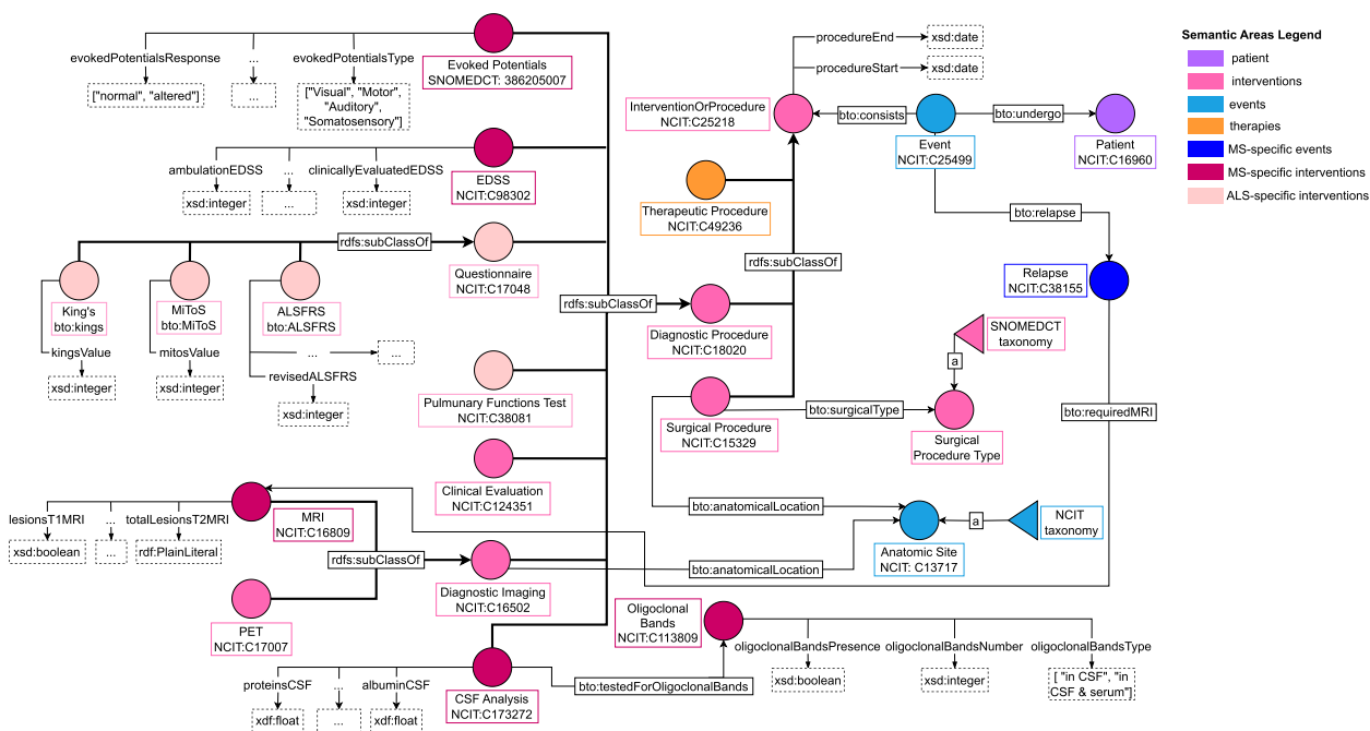
Fig. 6 “Intervention or Procedures” area, identified by the color pink. Classes in orange determine the “Therapeutic Procedures” area while we distinguish classes related to a specific disease with different colour tones. In particular, dark pink identifies classes related to MS whereas light pink ALS-specific classes. Class “Event” has 3 subclasses: surgical procedures, diagnostic procedures, and therapeutic procedures. Both surgical and therapeutic interventions are the same for MS and ALS patients while diagnostic procedures can differ based on the disease. See Table 9 for the legend
