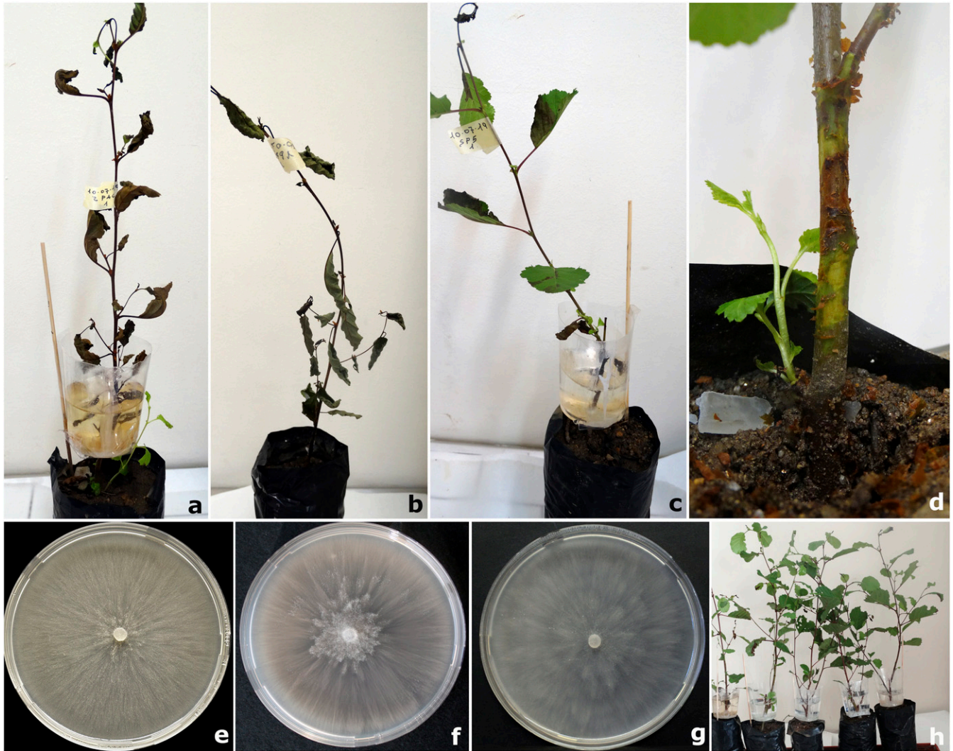
Figure S2. Symptoms observed on common alder seedlings 4 weeks after inoculation with Phytophthora acerina (a), Phytophthora plurivora (b) and Phytophthora pseudocryptogea (c). Necrotic lesion of the inner bark of the stem caused by P. pseudocryptogea (d). Colony morphology of P. acerina (e), P. plurivora (f) and P. pseudocryptogea (g) after 7 days growth at 20° C on carrot agar in the dark. Asymptomatic control seedlings (h).
