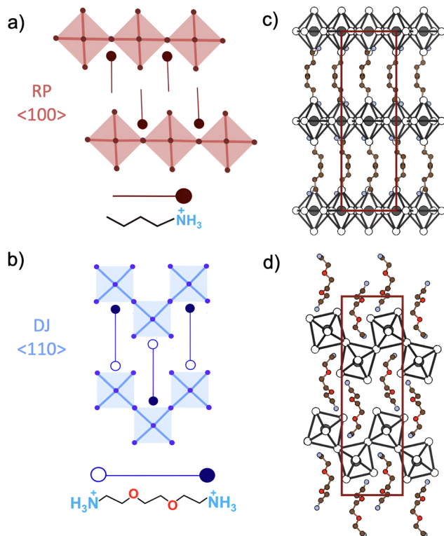
Fig. 1 Schematic representation of the flat \langle 100 \rangle -oriented Rudzlesden–Popper perovskite templated by BA + cations (a), and of the corrugated structure of the \langle 110 \rangle -oriented Dion–Jacobson perovskite templated by EDDBE 2+ cations (b); open and filled circles in the schematic ligand represent ammonium moieties with different coordination environments located at inequivalent crystallographic sites. The red and blue squares represent the individual PbI 6 4− octahedral units of the inorganic layers. (c) Crystal structure of BA 2 PbI 4 with space group Pbca (no. 61). (d) Crystal structure of (EDDBE)PbI 4 with space group P2 1 /c (no. 14). Both structures' b -axis has been aligned in the x -direction. The unit cells are highlighted in red, while H atoms have been omitted.
