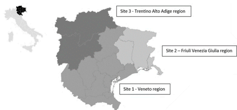
Figure 2. Map depicting investigated regions of North-eastern Italy.
