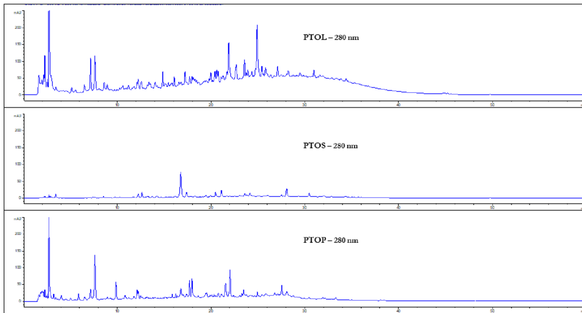
Fig. 1 Chromatograms of PT fractions from the three matrices (OL, OS and OP) obtained by HPLC–DAD at a wavelength of 280 nm (PT phytochemical fraction, OL olive leaves, OS olive stone, OP olive pomace)
