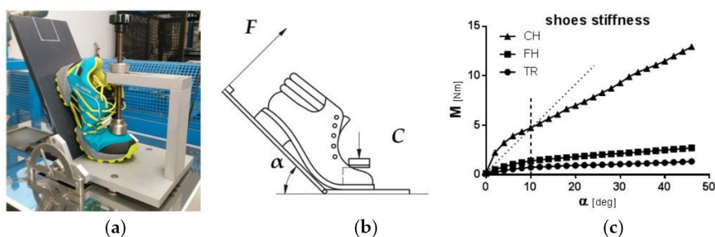
Figure 2. Bending test set-up (EN ISO 20344:2011): (a) stiffness bench test working; (b) schematic representation of the stiffness test. \alpha : bending angle; F : bending force; C : clamping force; (c) the bending angle \alpha is reported on the x-axis, whereas the corresponding bending moment M , coming from the bending force F , is shown in the y-axis. The secant relative to the CH footwear at 10 degrees is also plotted: its slope is the sole bending stiffness K_{Fs10}^{MTP} .
