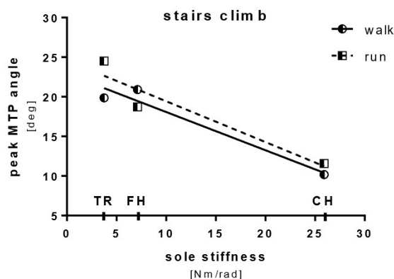
Figure 5. Results of the second campaign of data acquisition. Peak MTP angle versus shoe sole stiffness parametric in the speed of climbing of the stairs.
