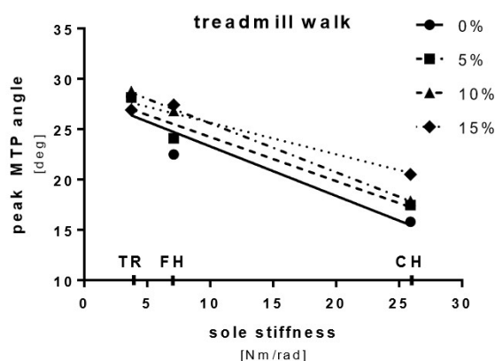
Figure 4. Results of the first campaign of data acquisition: peak MTP angle versus shoe sole stiffness parametric in the terrain slope for the walking trials.
