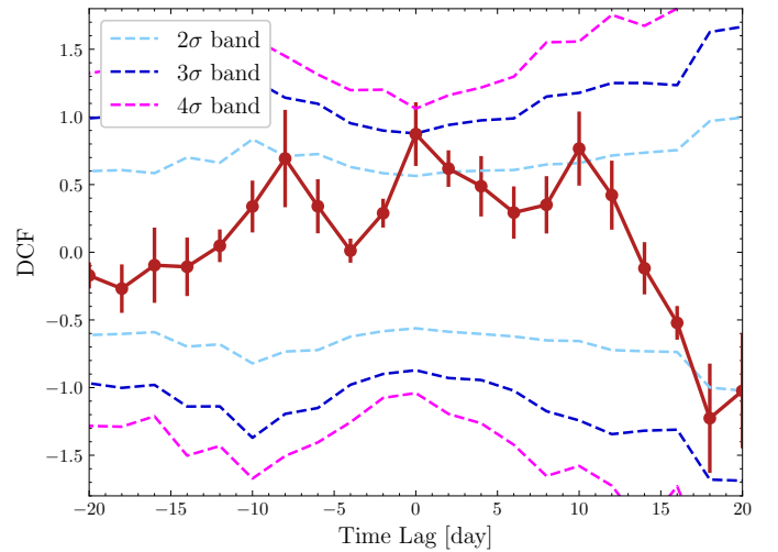
Fig. B.2. DCF computed for the MAGIC > 1 TeV and Swift-XRT 0.3-2 keV light curves between MJD 59700 (May 1, 2022) and MJD 59740 (June 10, 2022) with a time binning of 2 days. The red points are the obtained DCF values and their uncertainties. The light blue, dark blue and pink dashed lines show the 2\sigma , 3\sigma and 4\sigma significance bands, respectively (see the main text for more details).
