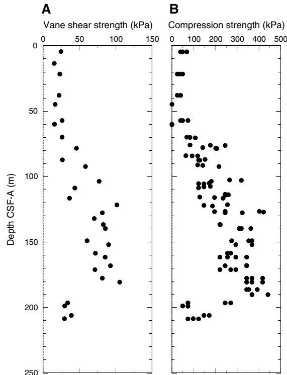
Figure F34. Strength, Site U1508. A. Shear strength measured by automated vane shear. B. Compressive strength measured using pocket and needle penetrometers.
