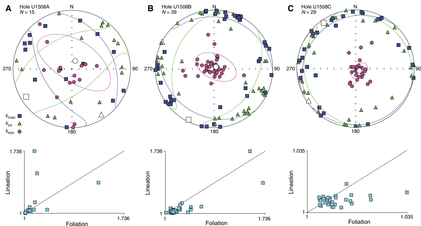
Figure F29. AMS data for discrete samples from (A) Hole U1508A, (B) Hole U1508B, and (C) Hole U1508C. Top: stereoscopic plots. Blue squares = \kappa_{max} axes, green triangles = \kappa_{int} axes, purple circles = \kappa_{min} axes. Mean directions of \kappa_{max} (open square), \kappa_{int} (open triangle), and \kappa_{min} (open circle) axes, shown along with their 95% confidence ellipses. N = number of samples. Bottom: corresponding lineation ( \kappa_{max}/\kappa_{int} ) vs. foliation ( \kappa_{int}/\kappa_{min} ) data from each hole.
