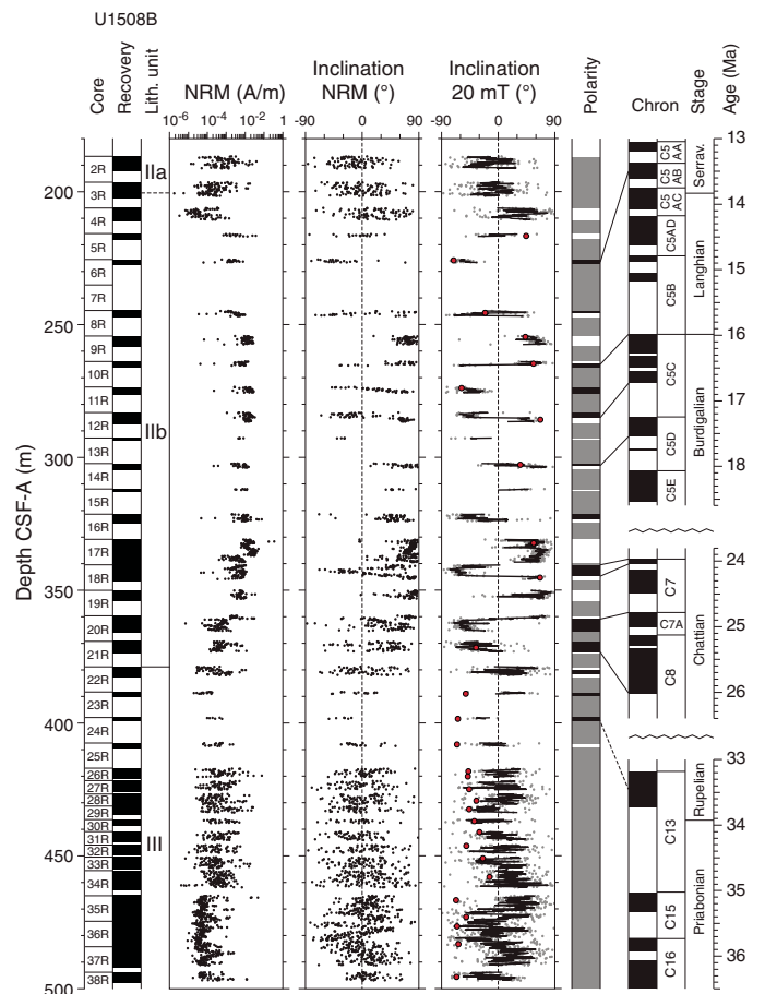
Figure F25. Pass-through paleomagnetic data, Hole U1508B. Black dots = NRM intensity and inclination, gray dots = inclination after 20 mT AF cleaning interpolated by 10-point moving average (black line), red dots = inclination from discrete sample analysis. Magnetic polarity: black = normal, white = reversed, gray = unidentified. Correlation with GPTS2012 is shown.
