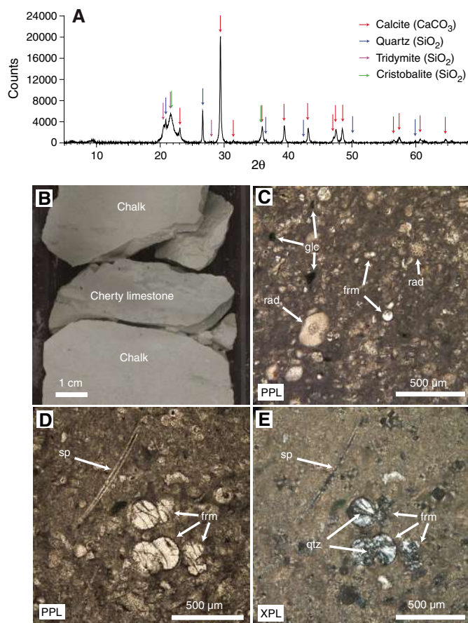
Figure F14. Detail of siliceous interval (371-U1508B-22R-1, 100–102 cm). A. XRD spectrum of homogenized cherty limestone with peaks of calcite and SiO 2 forms tridymite, cristobalite, and quartz identified. B. Cherty limestone interval between nannofossil chalk. C–E. Cherty limestone demonstrating foraminifers (frm), radiolarians (rad), glauconite (glc), sponge spicules (sp), and quartz (qtz) as foraminiferal chamber infill.
