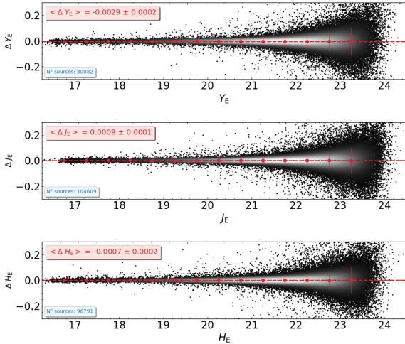
Fig. 19. Photometric differences between July and August observations of the self-calibration field for the Y_E , J_E , and H_E bands. The plots illustrate the photometric stability.
