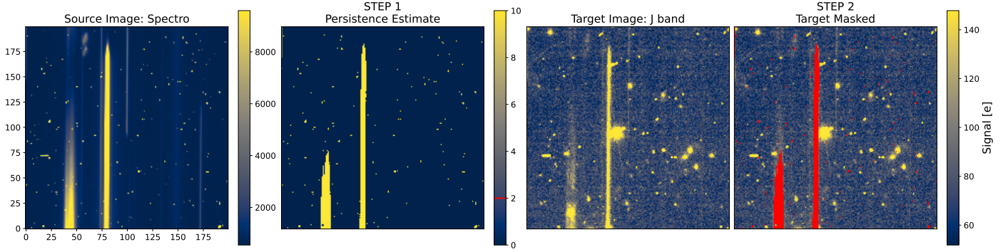
Fig. 5. Persistence masking scheme. In the first step, the persistence estimate is calculated using the persistence model applied to prior exposures (source images) for each target exposure. In the second step, the persistence estimates are thresholded to identify and mask pixels where the persistence charge exceeds 2e^- (indicated in red in the right image). Typically, the percentage of masked pixels does not exceed 2%.
