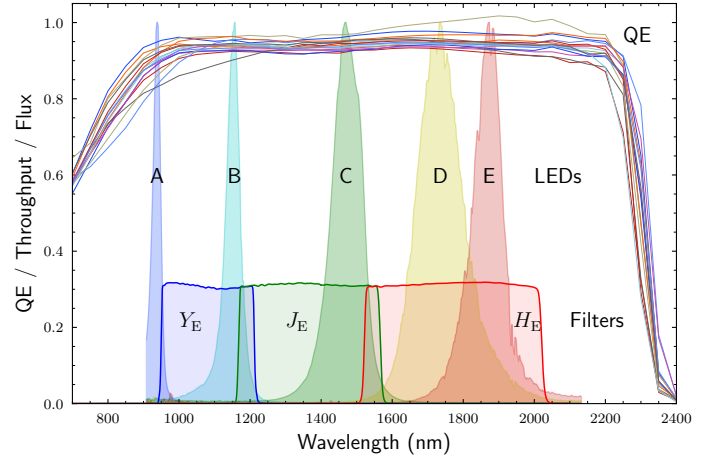
Fig. 8. Comparison of the average QE curves of the 16 NISP detectors, the normalised SEDs of the LEDs, and the Y_E , J_E , and H_E passbands (reduced by a factor of 3 in height to avoid cluttering near the top of the plot).
