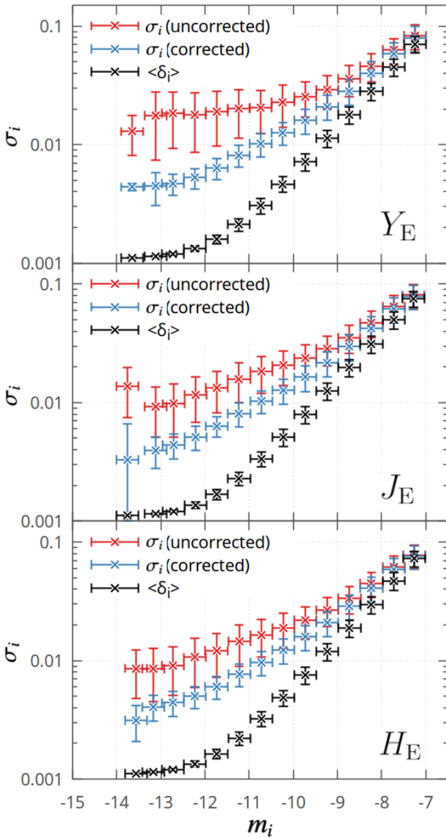
Fig. 11. Comparison of the scatter in magnitude from the repeated observations of the same source (‘uncorrected’ \sigma_i , red symbols), with the same scatter after the large-scale flat ( \sigma_i from Eq. (10), blue symbols), as a function of the instrumental magnitude m_i for the Y_E , J_E , and H_E filters. The averages of the photometric uncertainties for references (black symbols) are also shown. The scatter introduced by the large-scale non-uniformities is represented by the separation between red and black symbols, while the blue symbols represent the residual scatter after the application of the large-scale flat calibration.
