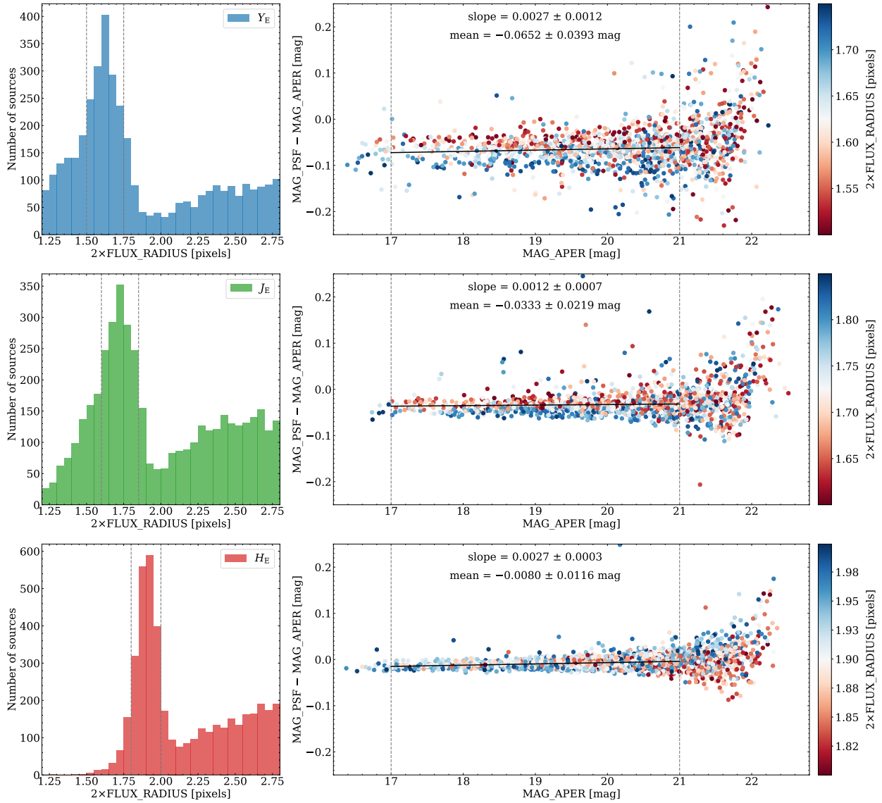
Fig. 14. Comparison between PSF-fitting and aperture photometry. Left column: Histograms of the half-light diameter for the three NISP passbands. The dashed lines indicate the ranges of point-sources plotted in the right panels and used by PSFex for PSF modelling. Right column: Difference between MAG_PSF and MAG_APER, colour-coded according to the half-light diameter. The mean difference and the slope of the linear regression (black line) for magnitudes between 17 and 21 (dashed lines) are also shown.
