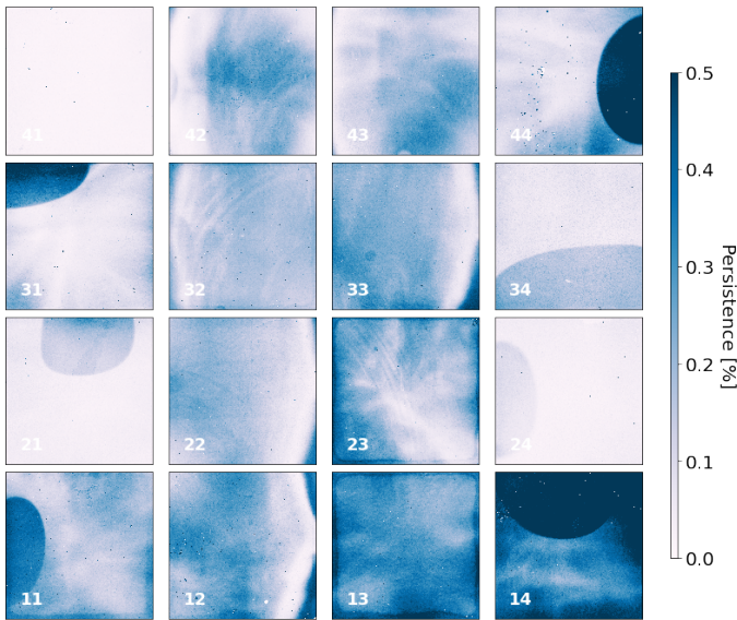
Fig. 4. Persistence signal accumulated during a dark exposure following an LED flat field illumination. The persistence is expressed as a percentage relative to the original flat field signal.
