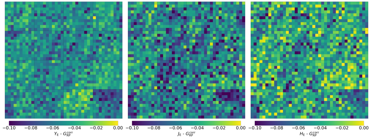
Fig. 18. FPA distribution of photometric residuals for sky patch 71 between Y_E , J_E , H_E , and Gaia photometry, after correcting for the colour term.
