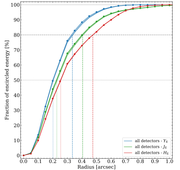
Fig. 13. Fraction of encircled energy as a function of the distance to the peak of the PSF profile. These curves were calculated using the same models shown in Fig. 12 for each of the 16 detectors of the three NISP passbands. The vertical and horizontal lines indicate the average radii encircling 50% (rEE50, dotted lines) and 80% (rEE80, dashed lines).
