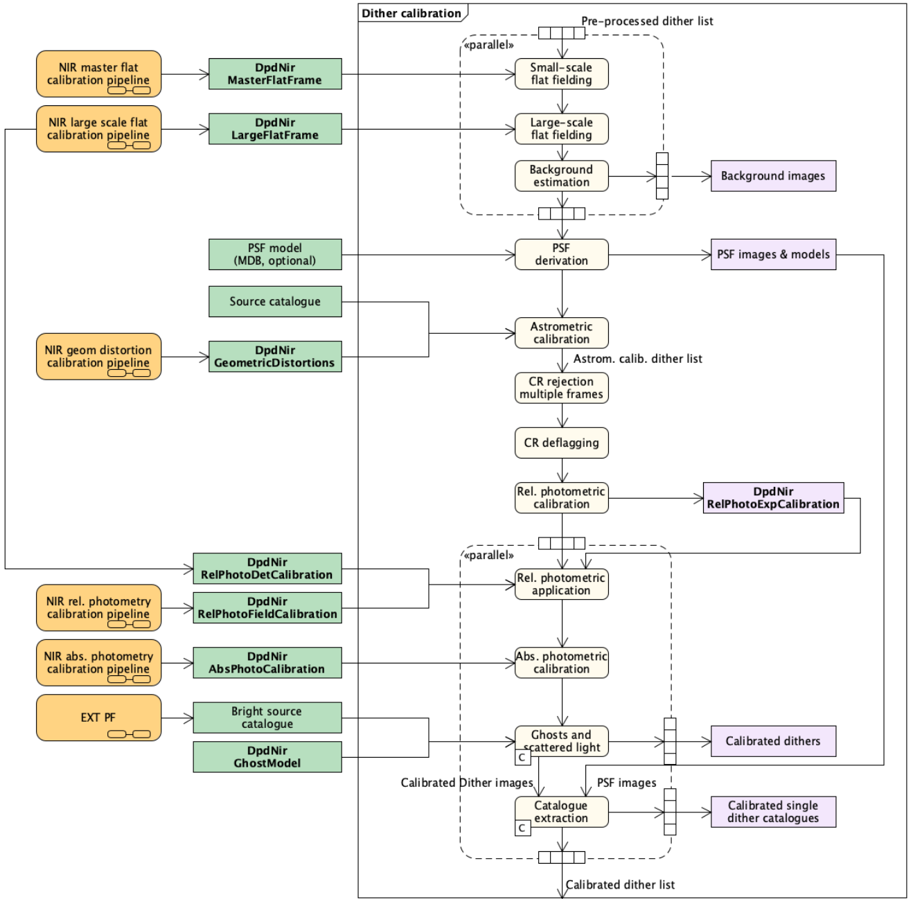
Fig. 7. NIR PF astrometric and photometric calibration PEs. Input products are shown as green boxes on the left. Some of them are taken from the MDB, while other products are generated by dedicated processing pipelines represented as orange boxes.
