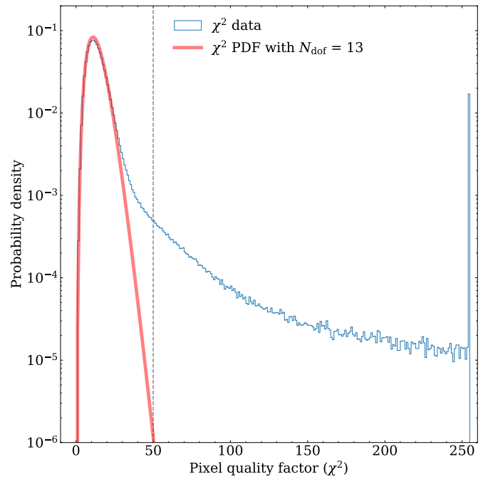
Fig. 6. Comparison between the PDF of the pixel quality factors ( \chi^2 ) for a spectroscopic MACC(15,16,11) exposure for one of the NISP detectors (blue histogram), and the PDF calculated for a \chi^2 distribution with N_{\text{d.o.f}} = 13 (red line). The threshold \chi^2 = 50 (dashed vertical line) distinguishes good- from bad-quality pixels. The \chi^2 value is encoded on-board as an 8-bit integer and thus has an upper limit of 255. Hence, the last bin corresponding to \chi^2 = 255 includes not only CRs, but all other pixels with a poor slope fit, such as bad pixels.
