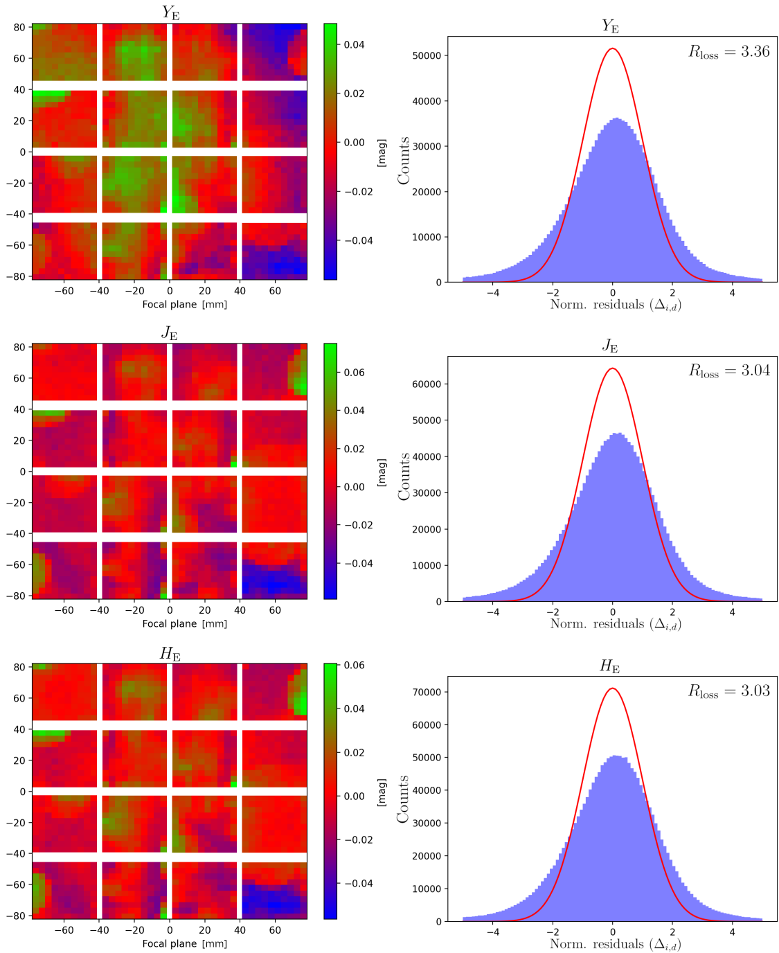
Fig. 10. Left column: Best-fit models of the Y_E , J_E , and H_E large-scale flats, \text{LSF}_d(x, y) , as in Eq. (7). Right column: Histograms of the normalised residuals of \Delta_{i,d}(x, y) from Eq. (8), compared to a normal distribution with mean zero and variance one (red curve). The quantity R_{\text{loss}} from Eq. (9) is reported in the plots.
