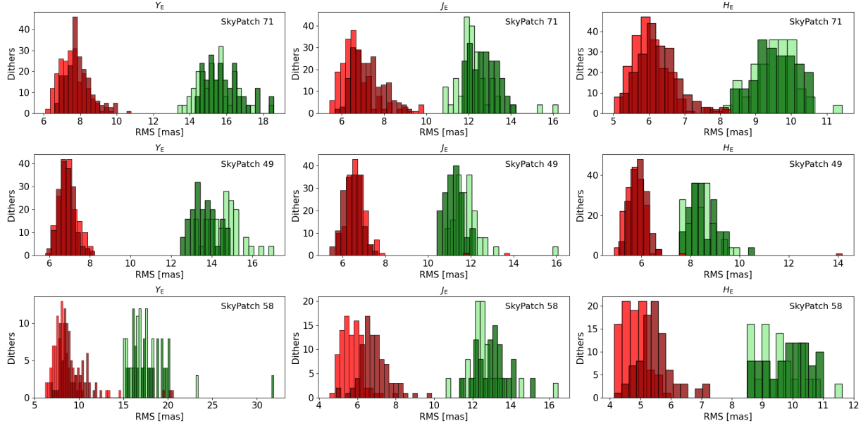
Fig. 16. Astrometric (RMS) residuals for dithers in the three Q1 sky patches. The green histograms are the residuals obtained from overlapping detections (required accuracy: 100 mas), while the red histograms illustrate residuals obtained through comparison with Gaia positions (required accuracy: 200 mas). The RMS for \Delta\alpha \cos(\delta) and \Delta\delta are represented by light and dark shading, respectively. The residuals are always well within the required accuracies.
