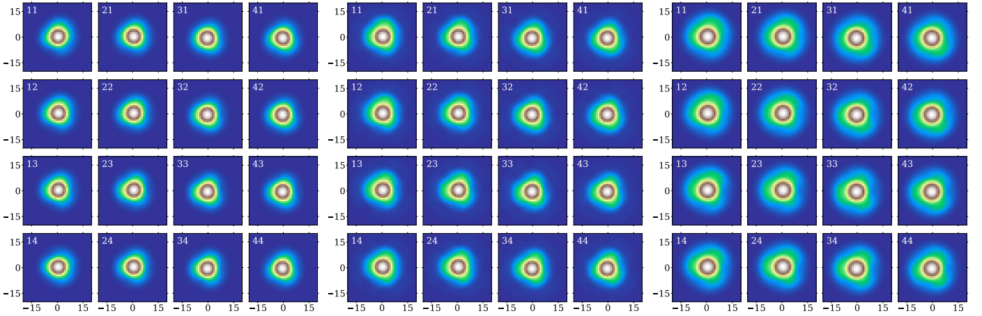
Fig. 12. 2D NISP PSF models derived from a typical EWS observation. The different panels are for Y_E (left), J_E (middle), and H_E (right) passbands and show the models (40 × 40 pixel stamps) derived for each of the 16 NISP detectors. The resolution here is 0''.05, subsampling the NISP pixel scale by a factor of 6.
