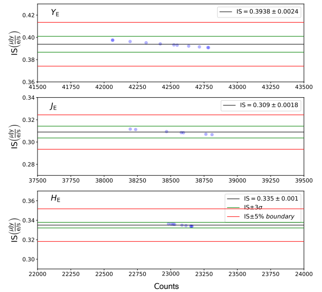
Fig. 15. Absolute flux calibration factor, IS , as a function of the observed counts, from the June 2024 WD calibration observations used for Q1. The observed counts were corrected for aperture losses. The black and green lines indicate the respective sigma-clipped mean of the individual IS measurements and the sample's 3\sigma uncertainty. The red lines denote the 5% requirement.
