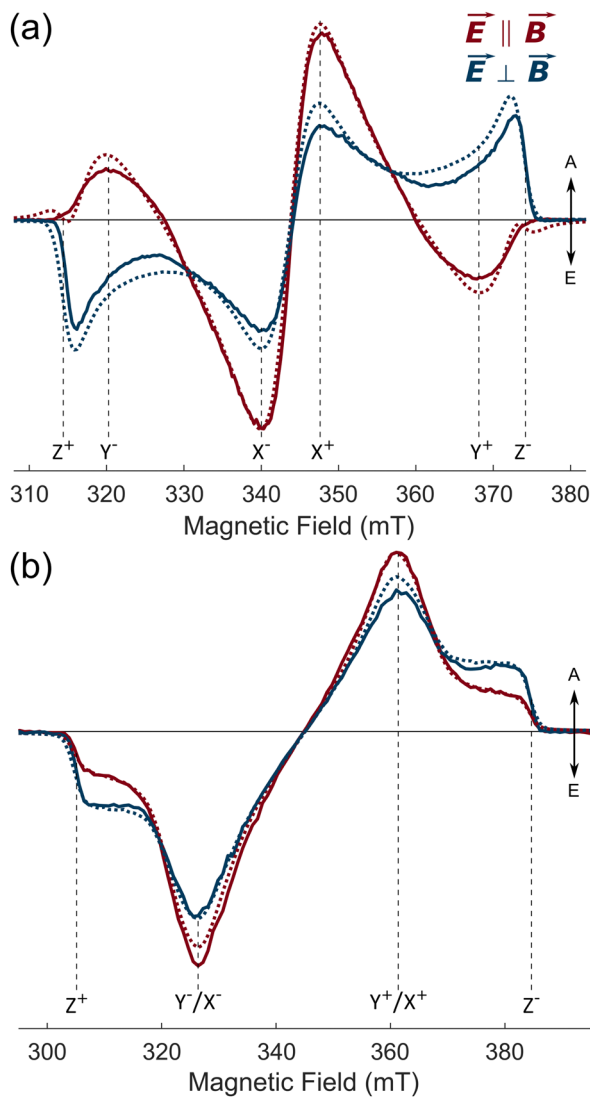
Fig. 5 Experimental (solid) and simulated (dashed) X-band transient EPR spectra of (a) PPor-OMe-PF 6 and (b) AlPor-OH in 3:1 MeTHF:CH 2 Cl 2 at 80 K and \sim 1 \mu\text{s} after the laser flash. The red spectra have been obtained with the electric field vector of the laser beam aligned parallel to the magnetic field of the EPR spectrometer; the blue spectra are with the electric field vector perpendicular to the magnetic field.
