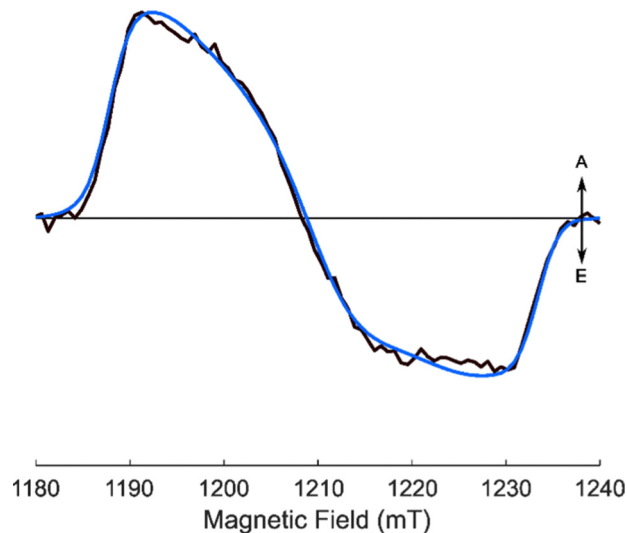
Fig. 6 Experimental and simulated Q-band transient EPR spectra of AlPor-O-PPor-PF 6 in 3:1 MeTHF:CH 2 Cl 2 at 80 K and \sim 1 \mu\text{s} ns after the laser flash ( \lambda_{\text{ex}} = 547 \text{ nm} ).
