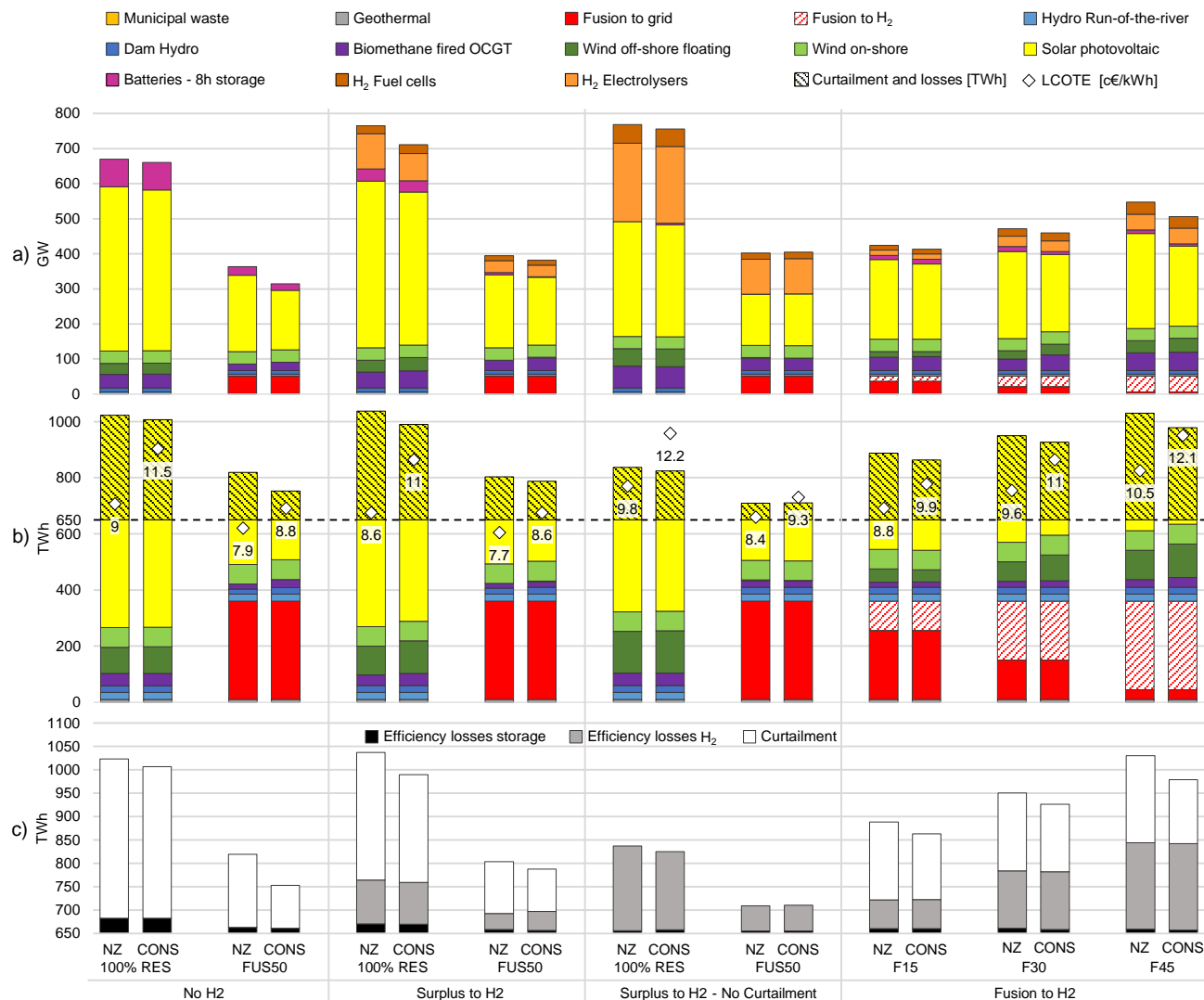
FIGURE 3. Optimization results for scenarios 100%RES and FUS50 in the four cases presented, in terms of a) power b) energy c) curtailment and losses. Results are shown both for the "Conservative" (CONS) cost option and the "Net Zero" (NZ) one. The total demand, equal to 650 TWh, is reported in dashed line.
