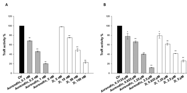
Fig. 5 TrxR inhibition. (A) TrxR1 activity was assayed by measuring the NADPH-dependent reduction of DTNB at 412 nm as described in the Experimental section. Error bars indicate S.D. (B) A2780 cells were incubated for 24 h with 2i or auranofin. Subsequently, TrxR activity was tested in cell lysates by measuring the NADPH-dependent reduction of DTNB at 412 nm. Error bars indicate S.D. * p < 0.05 ; ** p < 0.01 .
