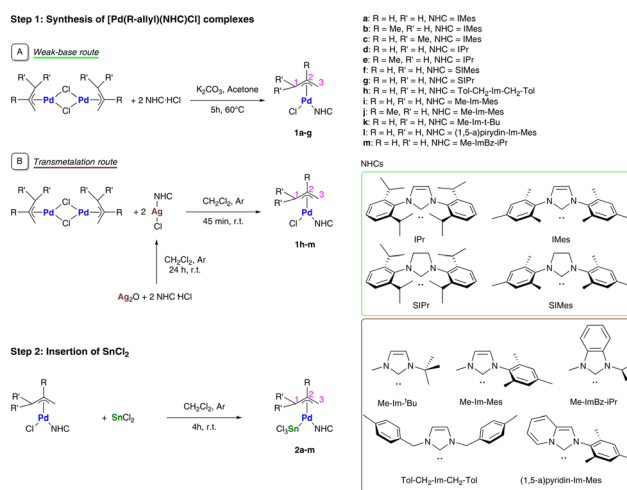
Scheme 1 Synthetic route to trichlorostannyl palladium–NHC allyl complexes.
