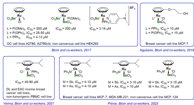
Fig. 1 Examples of trichlorostannyl complexes tested as anticancer agents. 50,52,54,55
