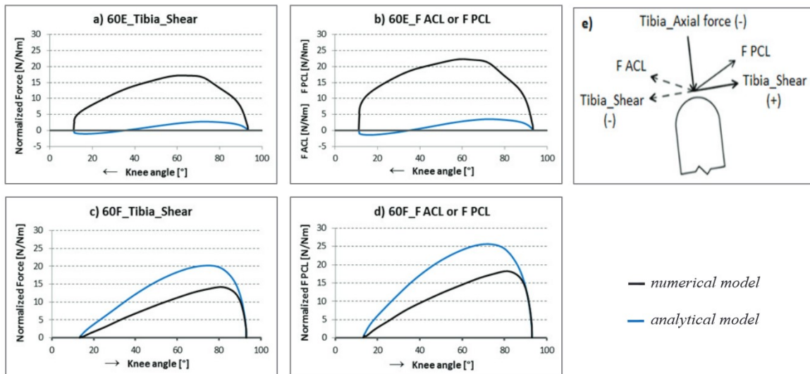
Fig.5. Knee loads at 60°/s from Numerical and Analytical solutions. a) Shear on Tibial Plateau (Tibia_Shear) in extension. b) Tension on ACL or PCL in extension, normalized to maximum knee torque. c) Shear on Tibial Plateau in flexion. d) Tension on ACL or PCL in flexion, normalized to maximum knee torque. e) Notation: shear positive if the force points forward. Tension at cruciates: shear positive, PCL strained. Shear negative: ACL strained.)
