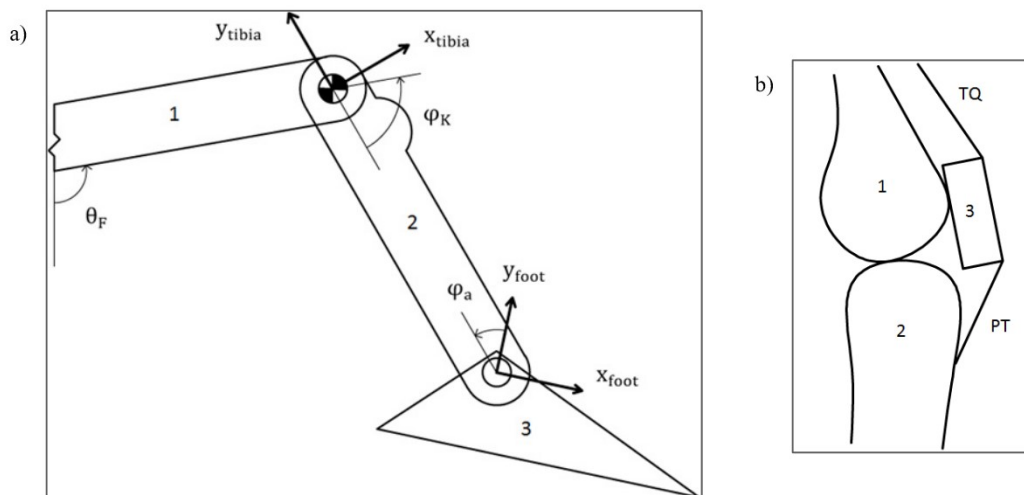
Fig.3. a) Analytical model used in the analysis. 1: femur; 2: tibia; 3: foot; \theta_F , \varphi_K , \varphi_a : kinematics angles; x_{tibia} , y_{tibia} , x_{foot} , y_{foot} : reference axis
