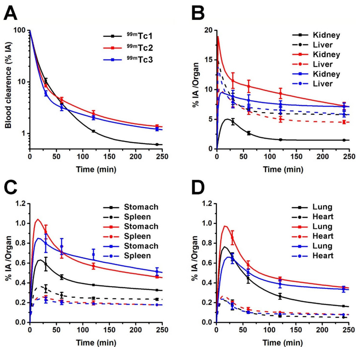
Figure 6. Time–activity curves in the main source organs: squares and circles show experimental data obtained from biodistribution studies after injection of 0.37 MBq of: ^{99m}\text{Tc}1 (black), ^{99m}\text{Tc}2 (red), and ^{99m}\text{Tc}3 (blue), respectively. The four individual graphs represent: (A) blood, (B) kidney and liver, (C) stomach and spleen, and (D) lung and heart. The lines depict the calculated time–activity curves.
