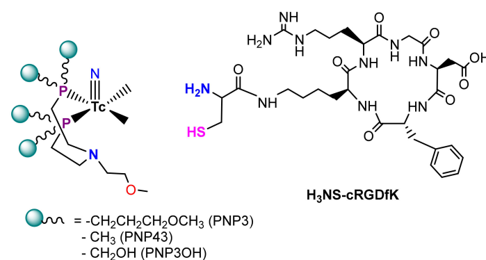
Figure 1. Left side: schematic drawing of the [ ^{99m}\text{Tc} ][Tc(N)(PNP)] synthons: PNP act as bidentate ligands, whereas the remaining two coordinative positions around the [Tc≡N] 2+ core are free for the coordination with a cysteine conjugated biomolecule. Right side: the cysteine-conjugated cRGDfK pentapeptide used in our experiments.
